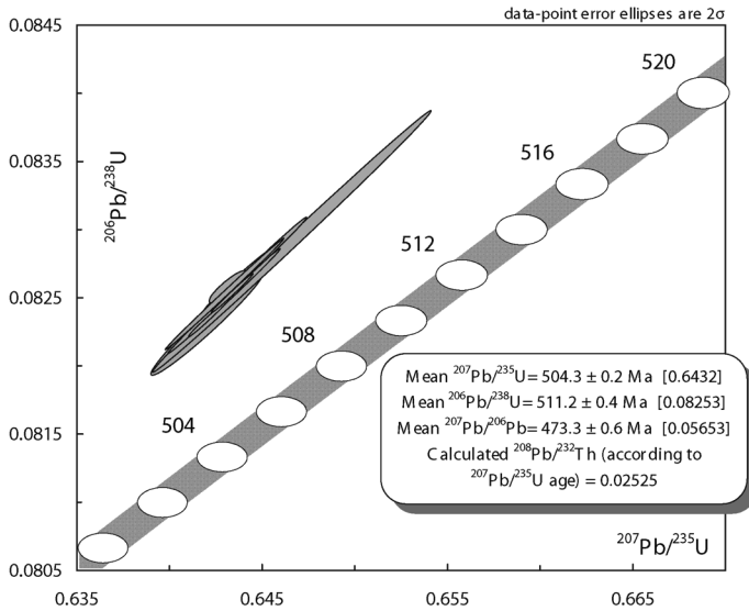
FIG. 6. – Concordia diagram of the Moacir standard. FIG. 6. – Diagramme Concordia du standard de Moacir.
