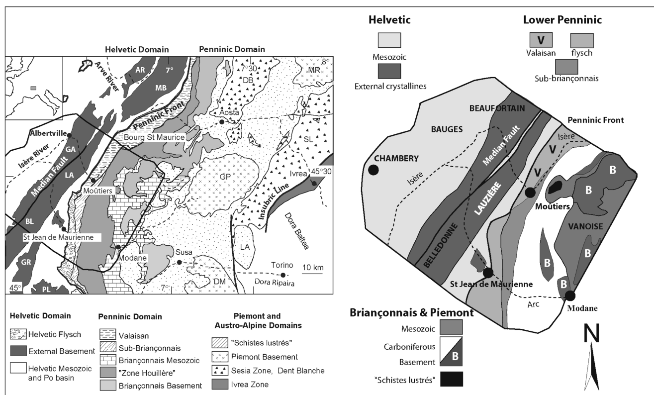
FIG. 1. – Geological setting of the Lauzière massif in the western Alps. Abbreviations : AR, Aiguilles Rouges; MB, Mont Blanc; GA, Grand Arc; LA, Lauzière; BL, Belledonne; GR, Grandes Rousses; PL, Pelvoux; ZHB, Zone Houillère Briançonnaise; GP, Gran Paradiso; DB, Dent Blanche; MR, Monte Rosa; SL, Sesia-Lanzo; LA, Lanzo massif; DM, Dora Maira.
