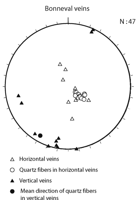
FIG. 5. – Stereograms of veins and quartz fibres from the Bonneval road area (area 2).
