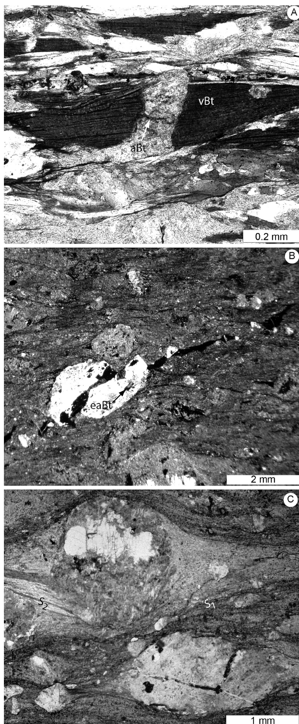
FIG. 3. – Microphotographs showing the deformation and recrystallisations in the Bonneval and Villar-Benoît formations. A: Bonneval-Tarentaise (area 2), broken old Variscan biotite (vBt) with recrystallisation of Alpine micro-biotite (aBt) in the tension gash. Another biotite crystal (bottom) is completely replaced by Alpine micro-biotite. B: Torrent du Tarlet (area 3). XZ section of a micro-conglomerate of the Villard-Benoît Formation: early alpine rotational deformation with recrystallisation of micro-biotite in the schistosity. Flakes of pre-Alpine biotite (eaBt) are preserved in the quartz clast. C: Bonneval (area 2), mylonite of the Bonneval Formation; the two Alpine schistosity planes are nearly parallel, S1 being outlined by micro-biotite. The younger schistosity (S2) is marked by sericite and oxides.
