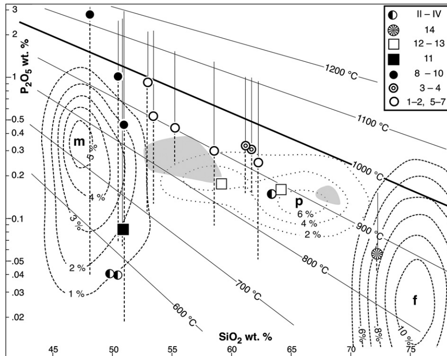
Fig. 9. P_2O_5 vs. SiO_2 with apatite saturation isotherms (after Harrison and Watson, 1984). Key to symbols as in Fig. 7a, sample numbers as in Table SM1 and Table 2. Vertical bars issued upward from each representative points join to the liquidus temperatures around 1100–1150 °C computed from each analysis (Sisson and Grove, 1993); downward dotted bars join to the zircon saturation temperature (Watson and Harrison, 1983).
