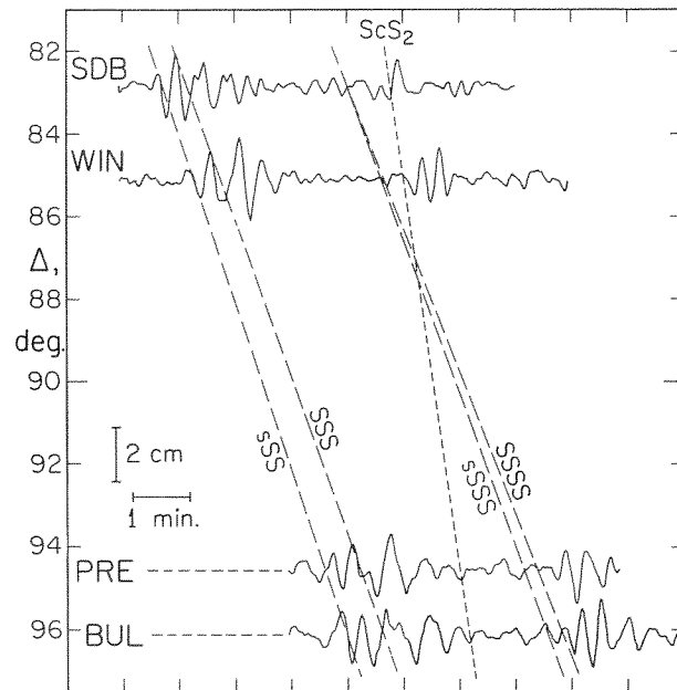
Figure 5 : EW seismograms for the 1965 event. All the instruments are 1500 gain Long Period WWSSN seismograms. The amplitude is given in centimeters. The origin time in the figure is 28 minutes after the earthquake. Arrival times calculated from JB tables are indicated for sSS, SSS, sSSS, SSSS and ScS_2 .
