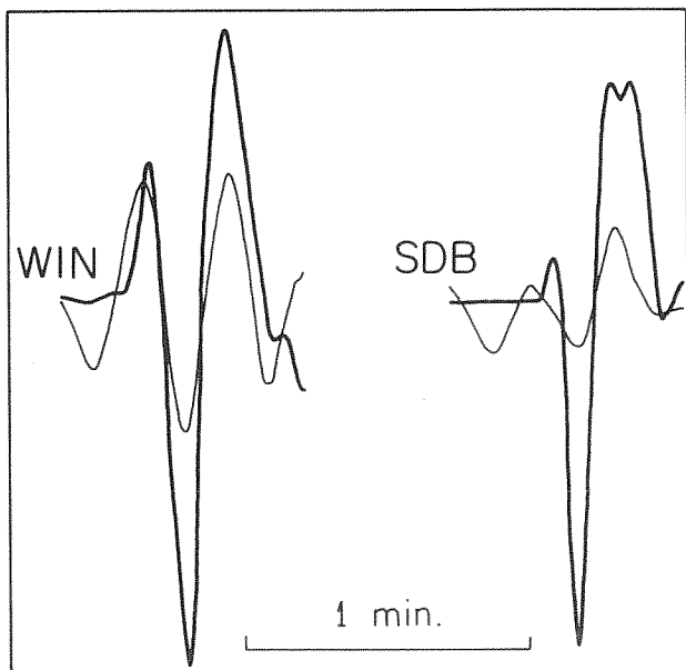
Figure 4 : Superposition of the 'S' (thick line) and ' ScS_2 ' (thin line) signals on the radial components at WIN and SDB using the time interval obtained from cross-correlation by Okal, 1978.
