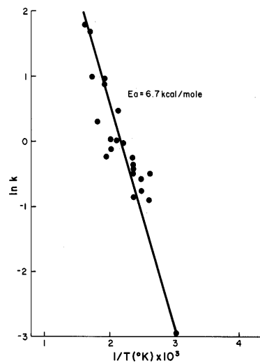
Fig. 7. Arrhenius plot of log (pseudo zero-order rate constant, k , far from equilibrium) vs. reciprocal temperature ( 1/K ) for calcite dissolution in the system CaCO_3-H_2O .
