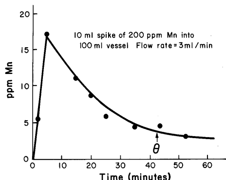
Fig. 3. Concentration of an inert tracer spike in the output stream of the CSTR reactor used for calcite and fluorite dissolution experiments. The position of the residence time, \theta , along the abscissa is noted.
