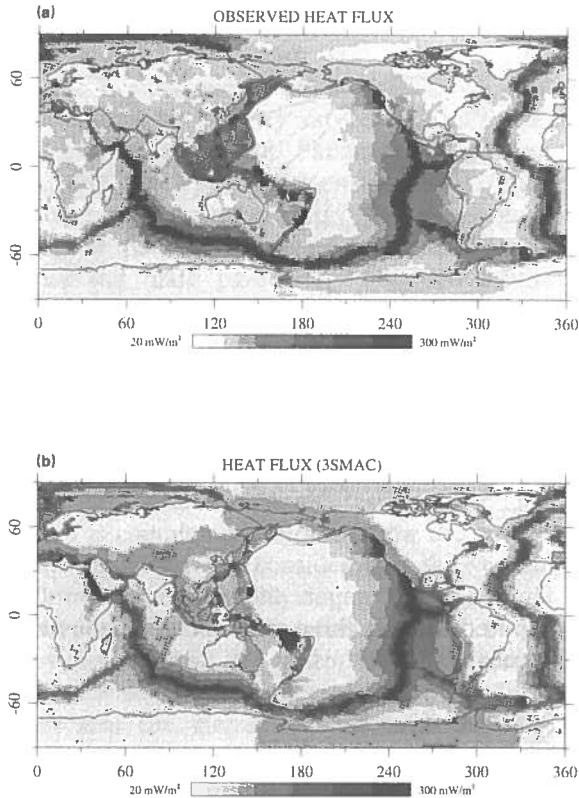
Fig. 7. Surface heat flux. (a) Observed, after Pollack et al. (1993). (b) Predicted from our 3SMAC model. The contour interval is 20 below 100 \text{mW m}^{-2} , and 50 above. Note the general agreement between the two maps.
