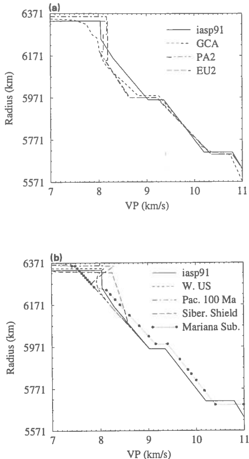
Fig. 12. Comparisons between our predicted seismic profiles in various regions with 'observed' profiles, for P-waves. The iasp91 model (Kennett and Engdahl, 1991) is plotted in both graphs. (a) 'Observed' seismic models: GCA (Gulf of California) from Walck (1984), PA2 (100 Ma Pacific Ocean) and EU2 (Eurasian shield) from Lerner-Lam and Jordan (1987). (b) Predicted seismic profiles in 3SMAC: they can be compared directly with the corresponding observed profiles. The profile 'Mariana Sub.' is for a subducting slab.
