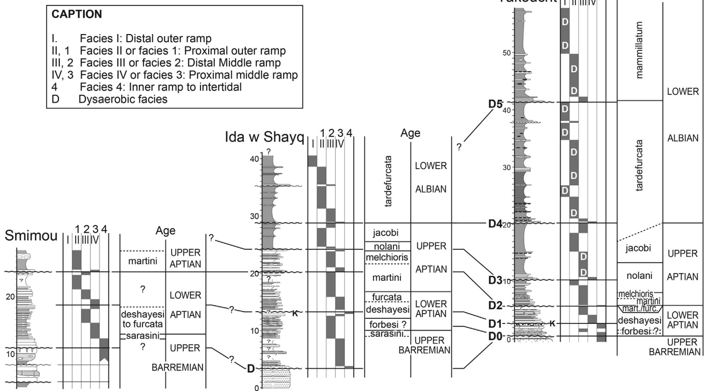
Fig. 10. East–West correlations of the Aptian–lower Albian sections in the northern part of the Essaouira–Agadir Basin. D: dysaerobic facies. See Fig. 3 for explanation of 1–4, and I–IV.
