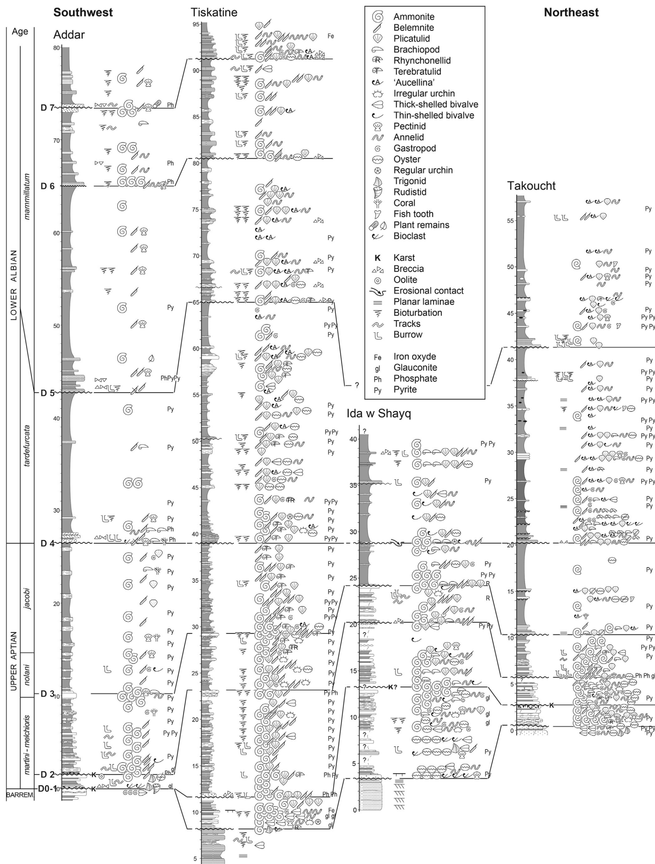
Fig. 5. North-South correlations of some Aptian–lower Albian sections of the Essaouira-Agadir basin.
