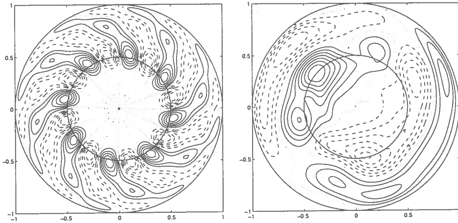
Fig. 1. Equatorial cross-section of the flow induced by an unstable viscous shear layer located at a cylindrical radius s = 0.5 in a rapidly rotating sphere. Two-dimensional numerical simulation assuming Proudman-Taylor invariance along the axis of rotation. Two polar caps ( s < 0.5 ) are rotating faster at \Delta\Omega + \Omega than the remaining part of the spherical boundary, which rotates at \Omega ( E = 10^{-5} ). Lines are contours of the stream function of the non axisymmetric flow. On the left, \Delta\Omega/\Omega = 0.033 gives a typical view of the flow at the onset of instability with a Rossby wave-type flow alike thermal convection. On the right, \Delta\Omega/\Omega = 0.1 yields a view of the nonlinear regime at 3 times critical. In that case the non-axisymmetric maximum velocity reaches 1/3 of its axisymmetric counterpart.
