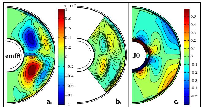
FIG. 4. (Color online) Meridional cross section contour maps showing orthoradial component ( \theta ) of emf \mathcal{E} and of electrical current \langle \mathbf{J} \rangle . (a) Averaged emf \mathcal{E}_t obtained from dns. (b) Reconstructed emf \mathcal{E}_{\alpha\beta} from inverted \alpha and \beta profiles. High latitudes (white area) are excluded from the least-square fit. (c) Mean electrical current from dns.
