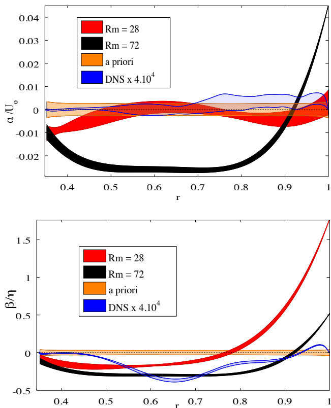
FIG. 2. (Color online) Radial profiles of the \alpha -effect (a) and \beta -effect (b) with their error bars, obtained by the inversion of DTS data for two magnetic Reynolds number: Rm = 28 and 72 . The a priori null profile, along with its error bar, is also drawn. The blue curve shows the \alpha(r) and \beta(r) profiles retrieved from a numerical simulation of the DTS experiment at Rm = 29 and Re = 2.9 \times 10^4 , blown up by a factor 4 \times 10^4 .
