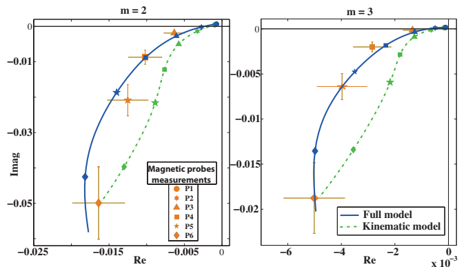
FIG. 3. (Color online) Measurements and model fits for an example of time-varying magnetic signals measured at 2f ( m=2 ) and 3f ( m=3 ) frequencies, for a rotation rate of the inner sphere f = -23\text{Hz} ( Rm = 72 ). See text for explanations.
