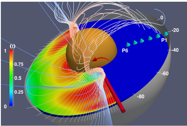
FIG. 1. (Color online) Sketch of the DTS experiment with its liquid sodium contained between an outer stainless steel shell (grey, with latitude labels in degrees) and an inner copper sphere (orange), which spins as indicated by the red arrow around the vertical rotation axis (here tilted for clarity). left half of the sphere : the field lines of the dipolar magnetic field imposed by the central magnet are drawn on top of the contour map of the fluid angular velocity \omega (normalized by that of the inner sphere) inverted from data measured for Rm = 94 . right half of the sphere : field lines of the total reconstructed magnetic field. The field lines are strongly distorted by the flow ( \omega -effect). The blue cones mark the radial positions of the 6 magnetometers P1 ( r = radius/r_o = 0.99 ) to P6 ( r = 0.50 ), which measure the azimuthal magnetic field. They can be placed at 4 different latitudes (here -20^\circ ).
