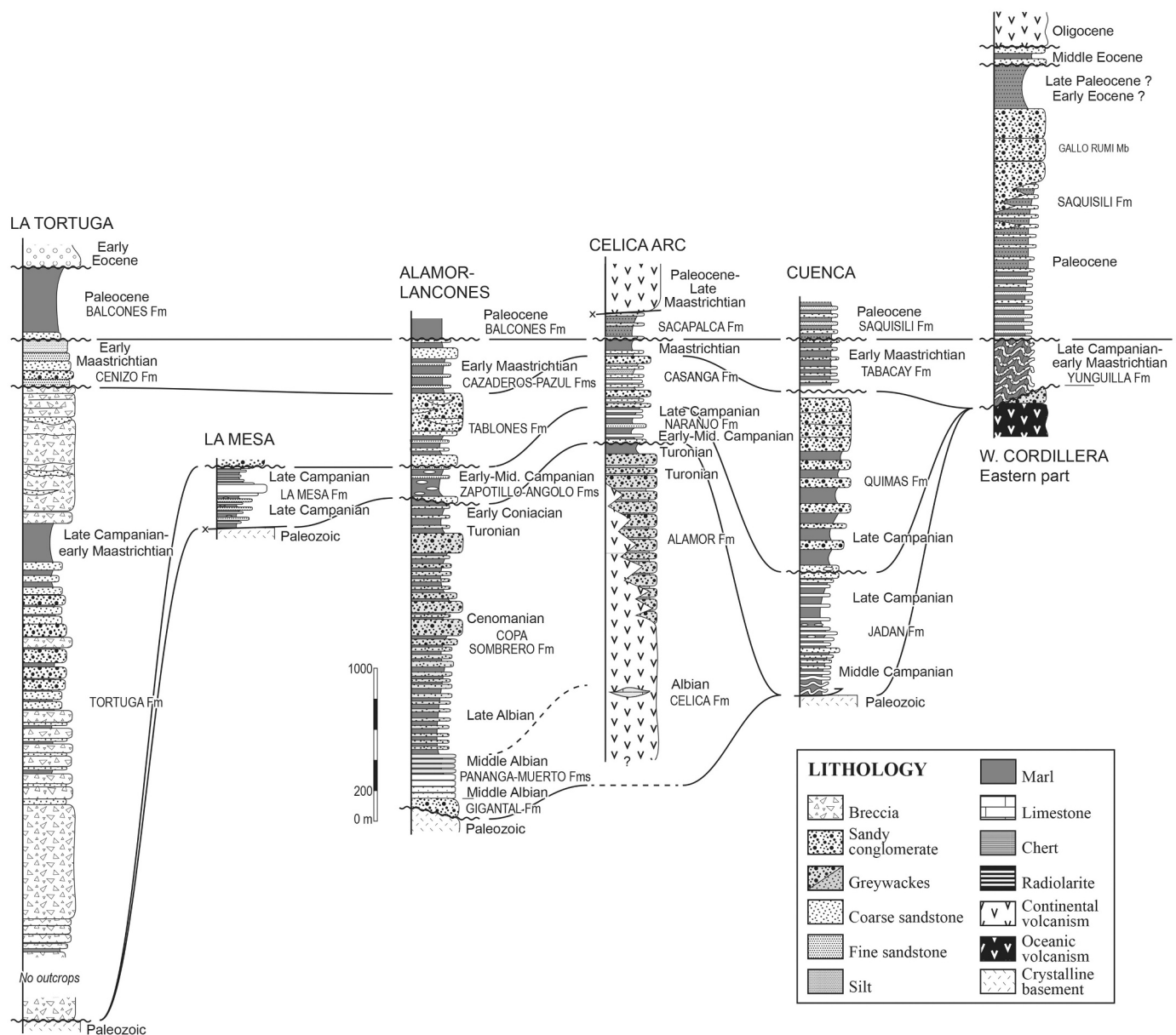
Fig. 3. Simplified stratigraphic succession of late Cretaceous-Paleogene age from the forearc zones of northwestern Peru (left) to central Ecuador (right) (from Jaillard et al., 1996, 1999, 2004, 2005).
