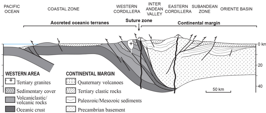
Fig. 11. Schematic cross section of the Ecuadorian Andes (adapted from Mégard, 1989). Note the western, west-verging wedge made of oceanic terranes, and the eastern, east-verging wedge, made of continental rocks. Compare with Fig. 6.
