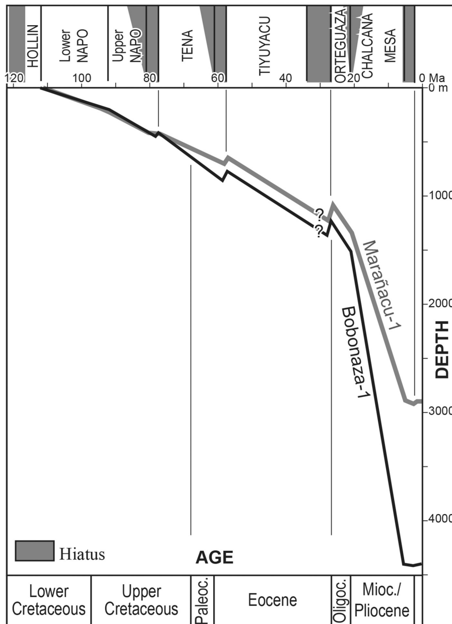
Fig. 9. Sedimentary accumulation in the Oriente Basin since the base of the Napo Fm (from Dashwood and Abbotts, 1990, simplified).
