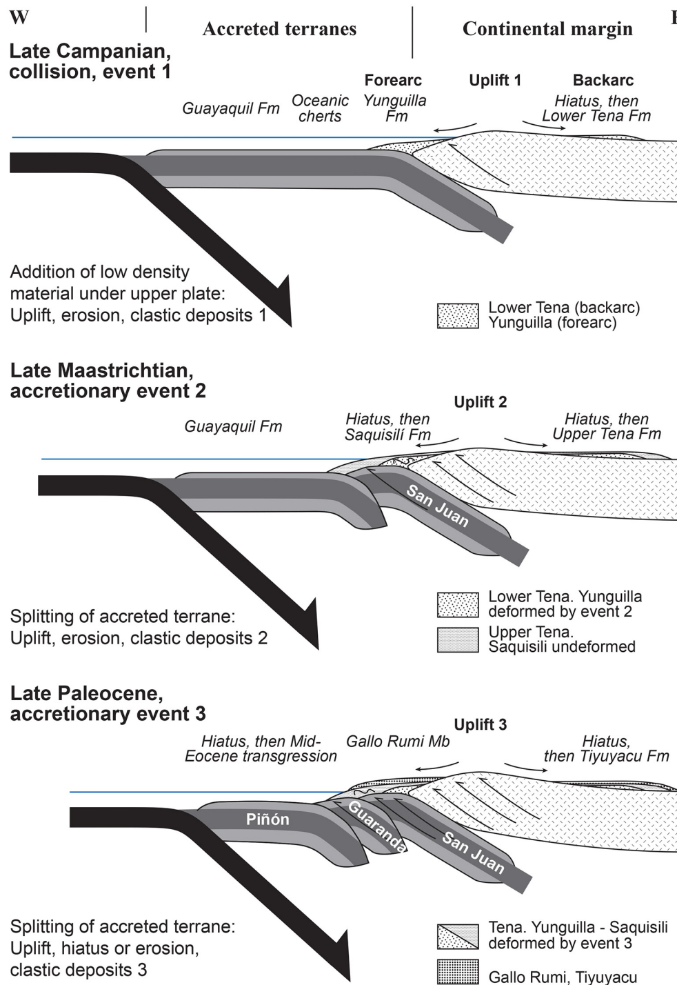
Fig. 13. Model for the accretion of oceanic terranes, accounting for the uplift, deformation, hiatuses and deposition observed in the forearc (accreted terranes) and backarc (Oriente Basin) areas of the Ecuadorian margin. The first accretionary event led to the end of the San Lorenzo island arc activity located on the accreted oceanic plateau. Arc volcanism resumed in latest Maastrichtian-Paleocene times, after accretionary event 2, on the continental margin.
