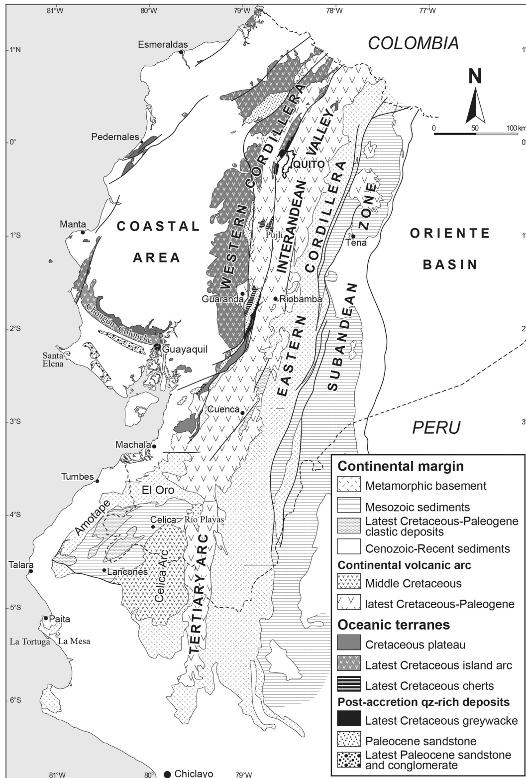
Fig. 1. Geological sketch of northern Peru and Ecuador, showing the main areas and localities cited in the text.
