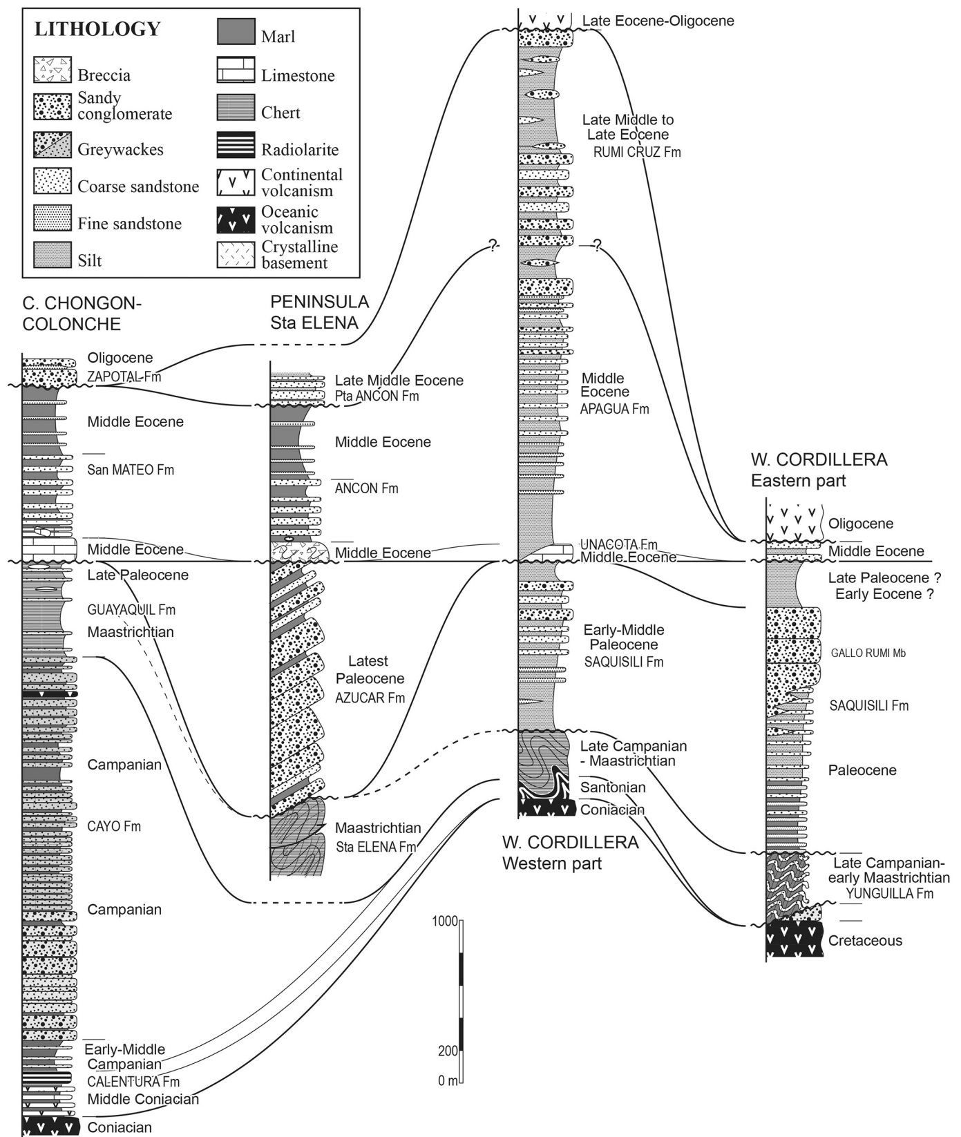
Fig. 4. Cretaceous-Paleogene successions of the accreted oceanic terranes, from Southwest Ecuador (left) to central Ecuador (right) (from Jaillard et al., 1995, 2004; 2009).
