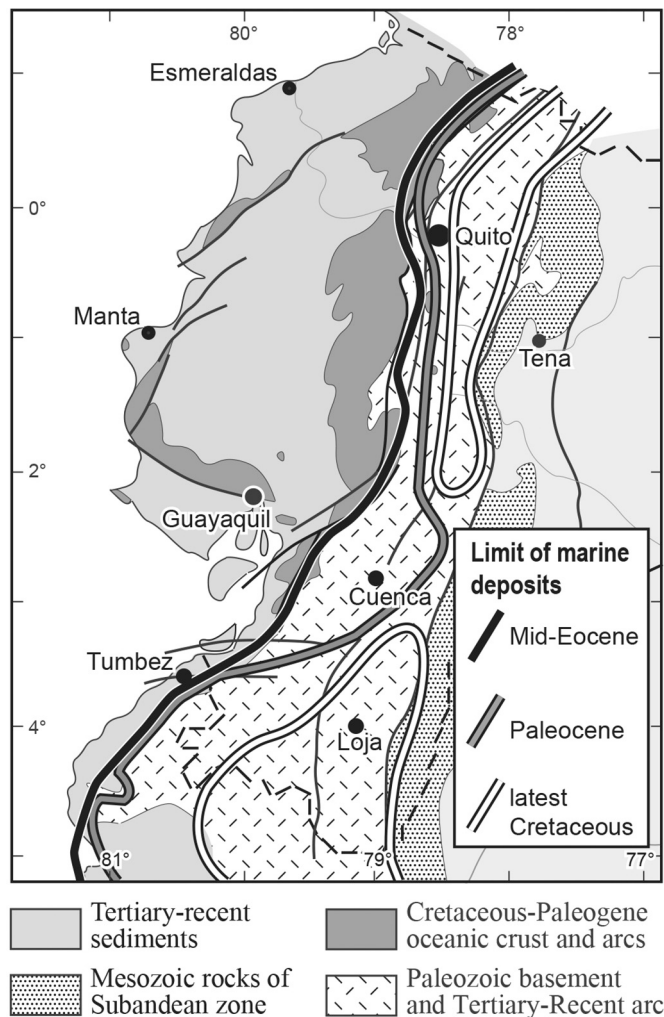
Fig. 7. Evolution of the marine shoreline from Maastrichtian to Late Eocene times (from Toro and Jaillard, 2005). Marine environment persisted on the oceanic terranes during this whole time-span, whereas most of the forearc zones and the Oriente Basin became emergent in latest Cretaceous and Paleocene times, respectively.
