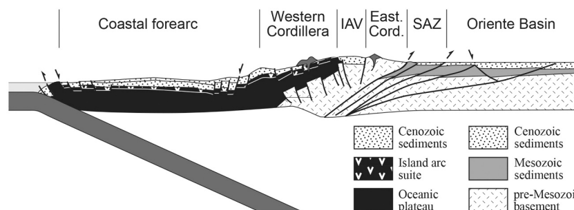
Fig. 6. Schematic cross section of the Ecuadorian Andes assuming the obduction of a single accreted terrane (simplified from Vallejo et al., 2019). Compare with Figs. 11 and 13. IAV: Inter-Andean Valley; SAZ: Sub-Andean Zone.
