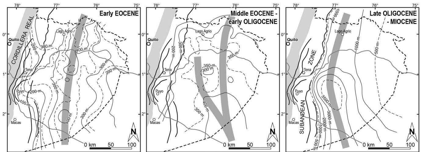
Fig. 10. Isopach maps of the Oriente Basin for various Tertiary periods (simplified from Christophoul et al., 2004). Grey line: depocenter axis.
