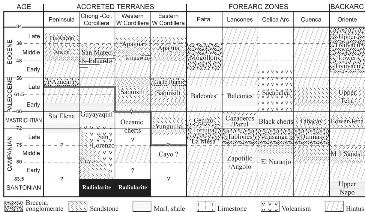
Fig. 5. Chronostratigraphic chart of the Late Cretaceous-Paleogene sediments deposited on the Ecuadorian margin. The grey bold line underlines the appearance of detrital quartz, and thus the accretion date of the described unit.
