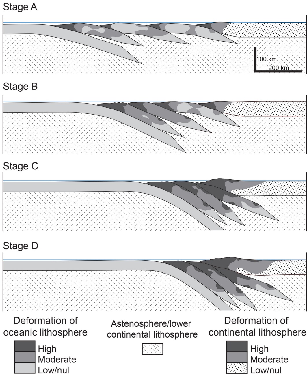
Fig. 12. 2D numerical modelling of the accretion of a low-density oceanic terrane divided by oblique, pre-existing faults (simplified from Bonnardot, 2003 ).
