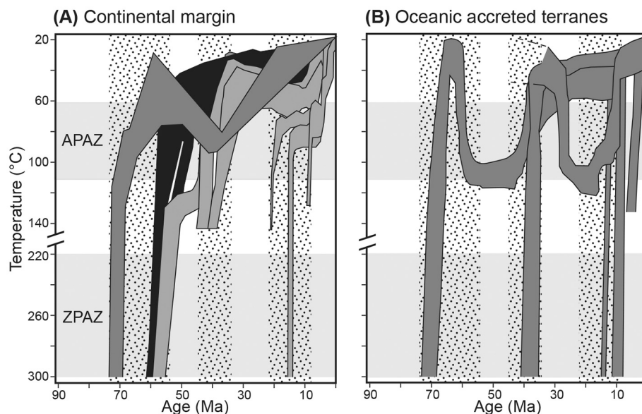
Fig. 8. Thermal history of the Ecuadorian Andes (after Spikings et al., 2010). Dotted areas: inferred exhumation periods. (A): Continental margin. Light grey: northern Eastern Cordillera; black: southern Eastern Cordillera; dark grey: Amotape Massif. (B) Oceanic accreted terranes (Western Cordillera). APAZ and ZPAZ: Apatite and Zircon partial annealing zone, respectively.
