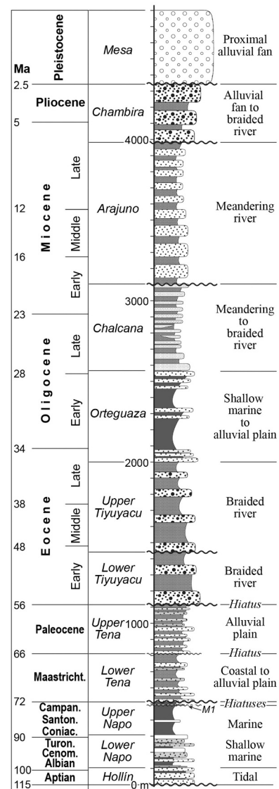
Fig. 2. Composite and simplified series of the Oriente Basin, Ecuador (compiled from Jaillard et al., 1997; Christophoul et al., 2004; Vallejo et al., 2021).
