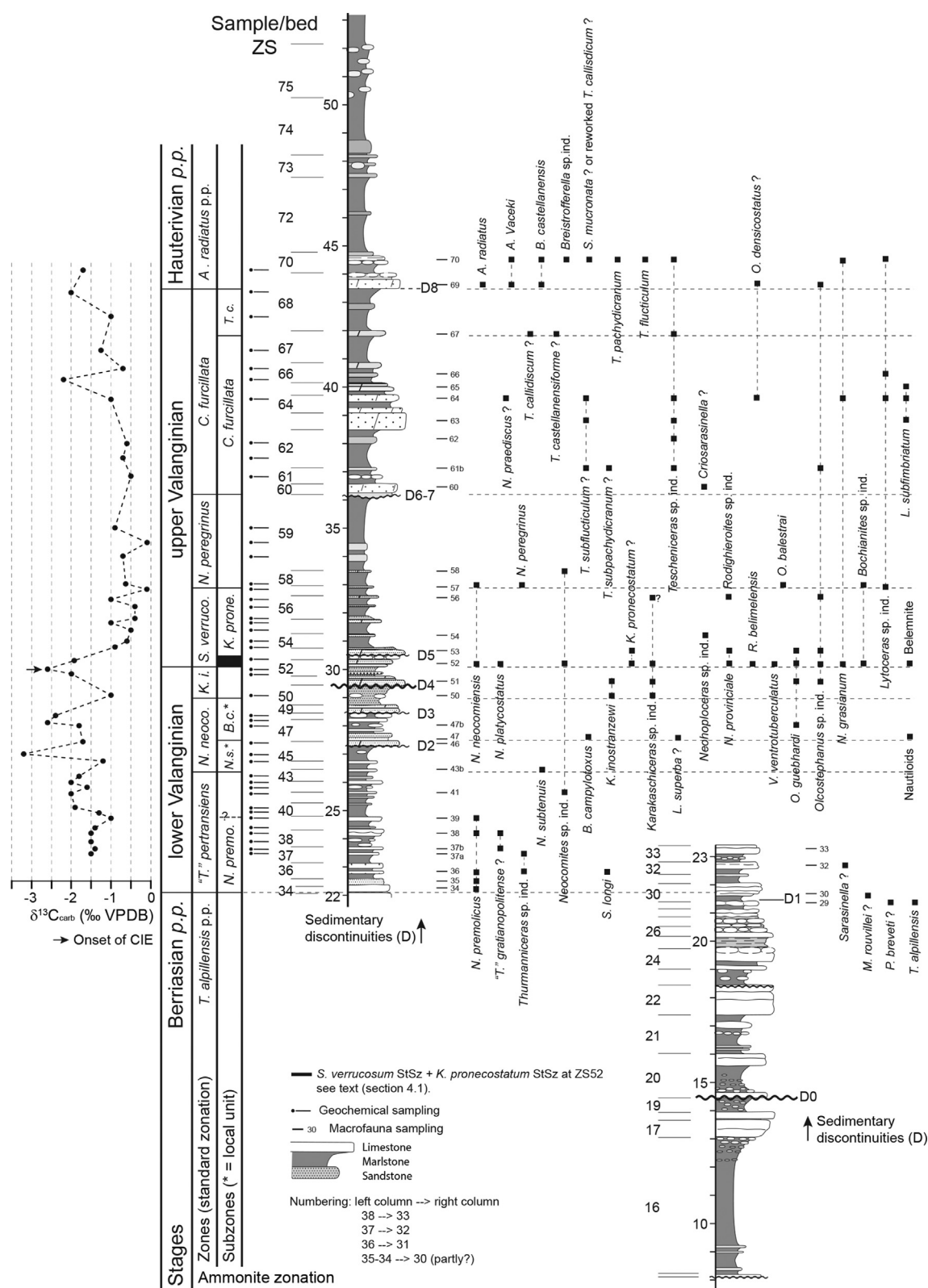
Fig. 5. The Zaouia Sidi Abderahmane section (two outcrops). Stratigraphic distribution of macrofauna (mainly ammonites; a question mark is added when identification is doubtful) and ammonite zonation (standard and local units); layers of sampling are indicated at the right of the succession. Sedimentary discontinuities (D). Carbon isotopic curve; layers of sampling are indicated at the left of the succession.
