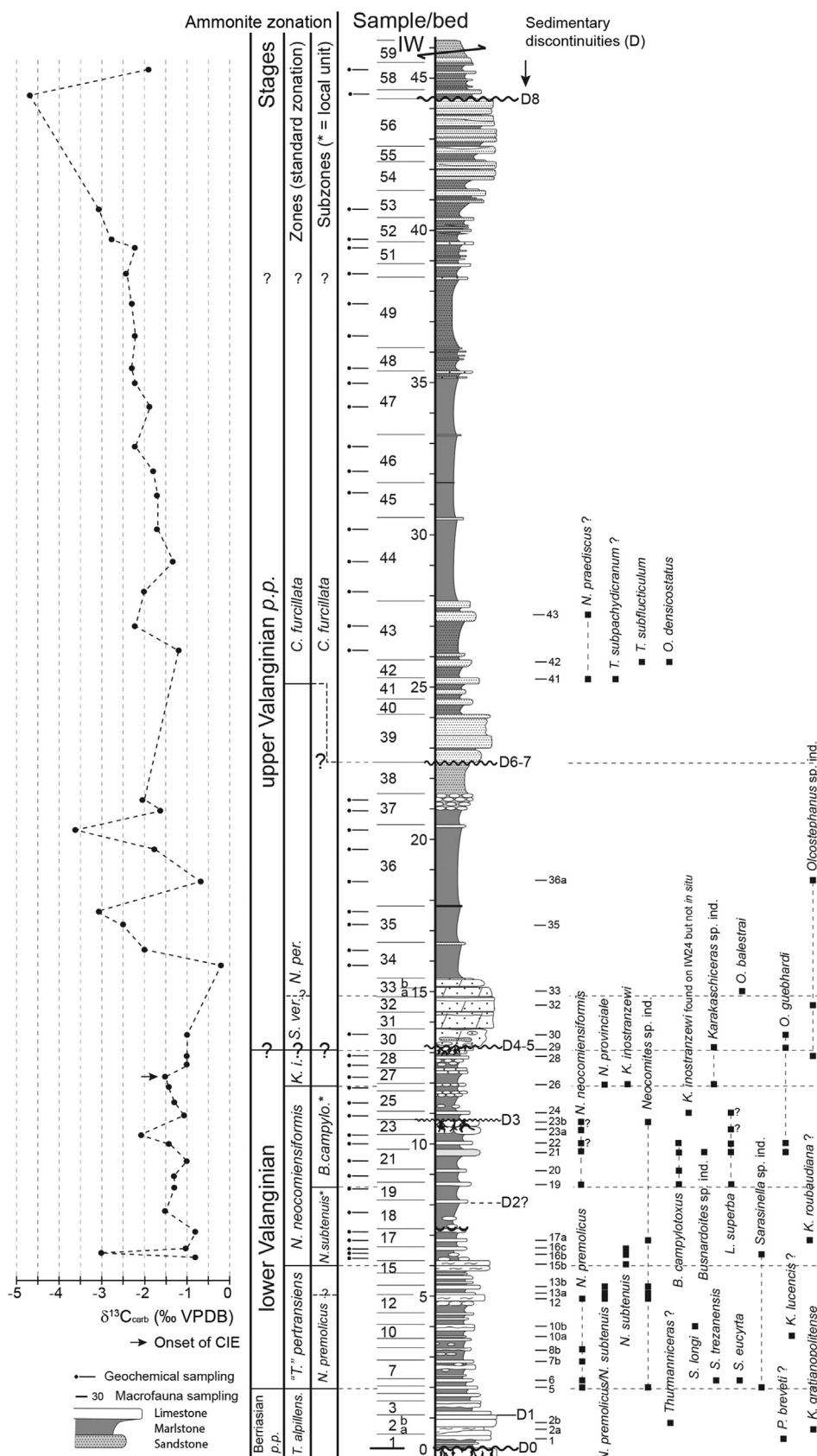
Fig. 7. The Ida w lldar section. Stratigraphic distribution of macrofauna (mainly ammonites; a question mark is added when identification is doubtful) and ammonite zonation (standard and local units); layers of sampling are indicated at the right of the succession. Sedimentary discontinuities (D). Carbon isotopic curve; layers of sampling are indicated at the left of the succession.
