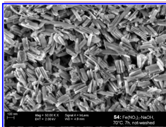
Figure 9. FESEM micrograph showing low acicular goethite (S4) synthesized from the water- \text{Fe}(\text{NO}_3)_3\text{-NaOH} system at 70^\circ\text{C} .
