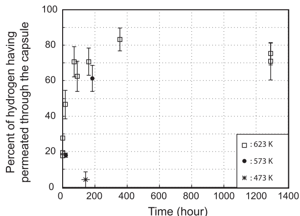
Fig. 4 – Percentage of hydrogen having permeated through gold as a function of time in experiments on acid oxalic decomposition at three different temperatures. Note that at least 20% of the initial hydrogen remained after 1300 h in the gold capsule at 350 °C.
