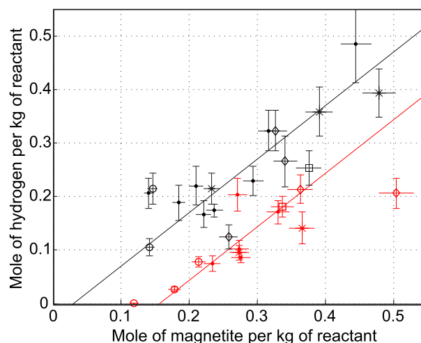
Fig. 9 – Relationship between the quantities of magnetite and hydrogen (estimated using magnetism and chromatography, respectively) produced in experiments using BOF/CBOF (black) and CARBOF (red) as starting materials. (For interpretation of the references to colour in this Figure legend, the reader is referred to the web version of this article.)
