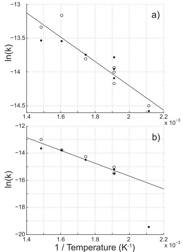
Fig. 11 – Arrhenius plots of the kinetic constant for the experiments using CBOF (a) or CARBOF (b) as starting materials. The constants of the reaction (5) ( k in s^{-1} ) were determined by fitting a first order kinetics to the reaction progress vs. time curves. The reaction progresses were derived from the amount of produced hydrogen (dots) or from the amount of produced magnetite (open circle). The plain lines are the fits used to derive the activation energies. For experiments using CARBOF as starting material (b), the experiment at 473 K (COLACE116) was not used for the fit because its reaction progress is close to zero and its error has too much weight on the derived activation energy value.
