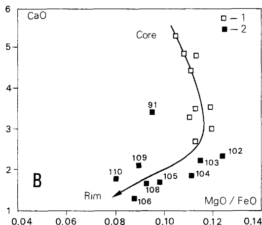
Fig. 5. CaO versus MgO/FeO diagrams from garnets: 5a – Sample GO 77a – (1) from the core; (2) from the rim. 5b – Sample GO 77b – (1) from the core; (2) from the rim.
