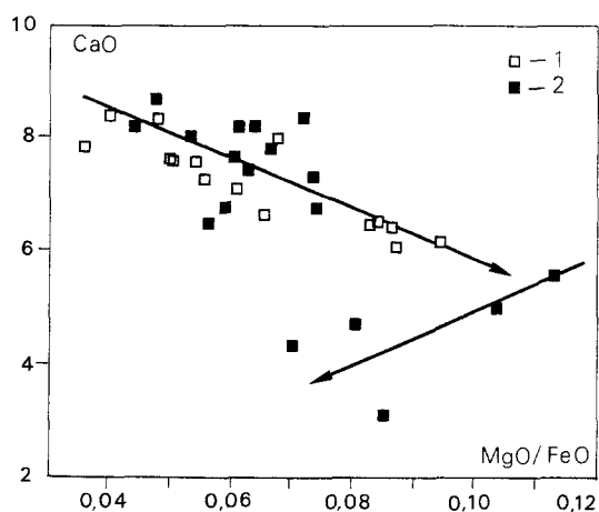
Fig. 6. CaO versus MgO/FeO diagram for sample GO 76b: (1) from the core of the main crystal; (2) from the rim of the main crystal and from small grains scattered in biotite.
