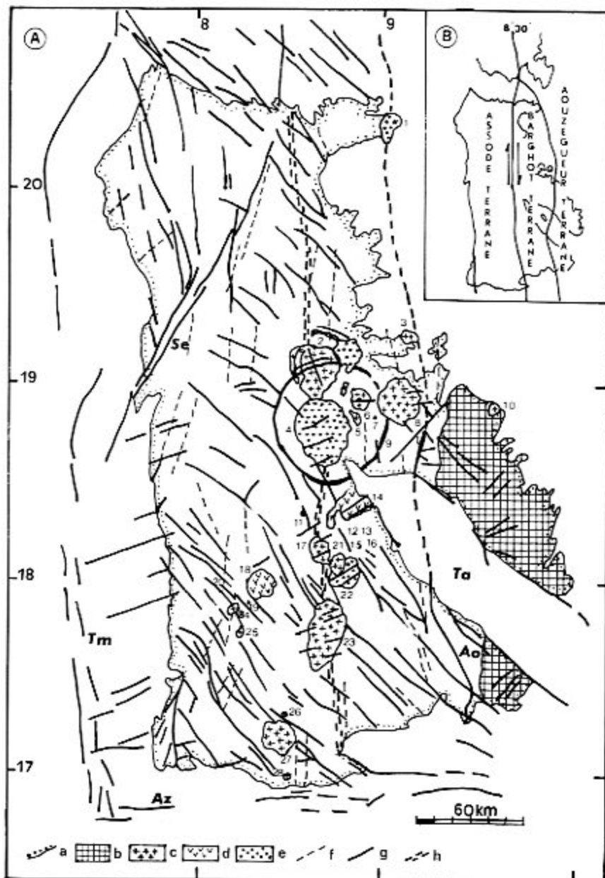
Fig. 2. (a) Geological sketch map of Air. a = geographical limit of the Air massif; b = Proche-Ténéré Formation; c = Taghouaji type ring complexes; d = Goundaï type ring complexes; e = Ofoud type ring complexes; f = foliation trend in gneissic basement; g = lineaments and faults; h = Raghane shear zone; Ao = Aouzegueur belt; Az = Agadez Town; Se = Serchouf lineament; Ta = Tâfidet graben; Tm = Tim Mersoï basin. The Air ring complexes are numbered from 1 to 28 (see Table 1 for description and explanation). (b) Air terranes (after Liégeois et al., 1994).
