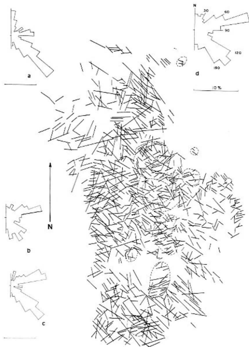
Fig. 4. Map of the lineaments in the Air massif. Rose diagrams represent cumulative lengths of lineaments in (a) the northern, (b) the central and (c) the southern parts of the massif and (d) in the entire massif.
