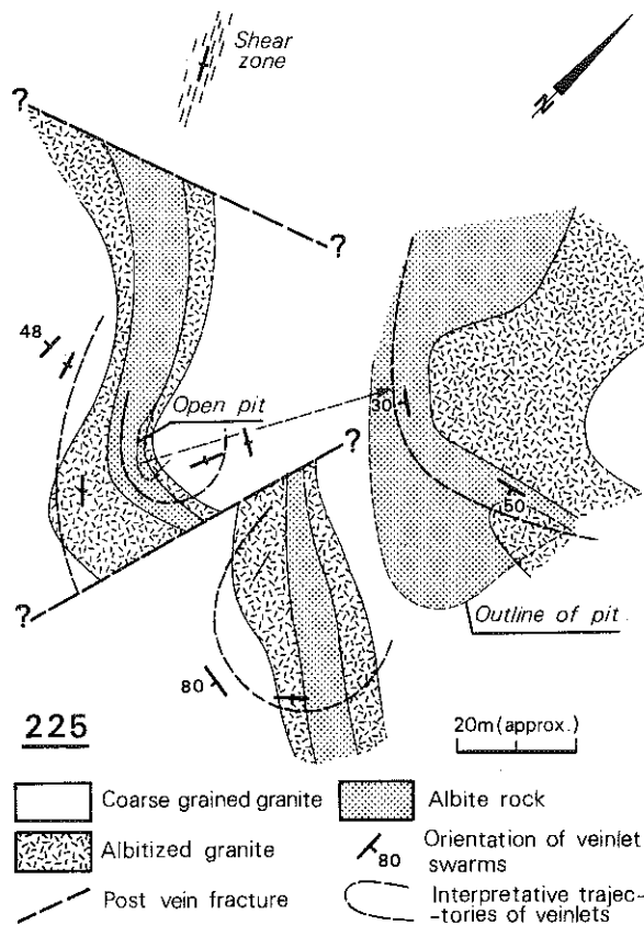
Fig. 3. Map of the 225 deposit showing the curvilinear shape of the albitite zone flanked by albitized granite and the orientation of the veinlets.
