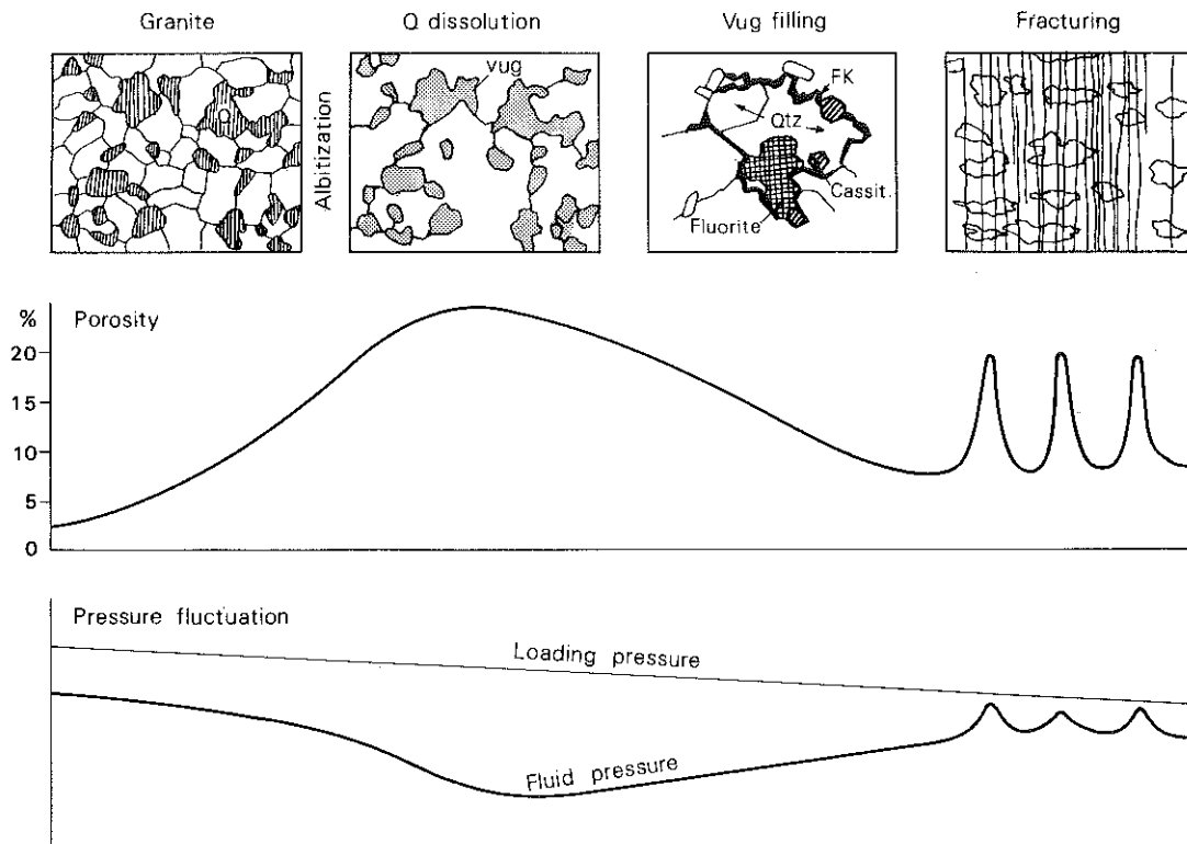
Fig. 11. Cartoon showing an interpretative hydrothermal scenario for the Emuford district and the expected correlation between textures and qualitative estimates of permeability and fluid pressure variability. The decreasing slope of the load pressure is attributed to the erosion above the pluton.
