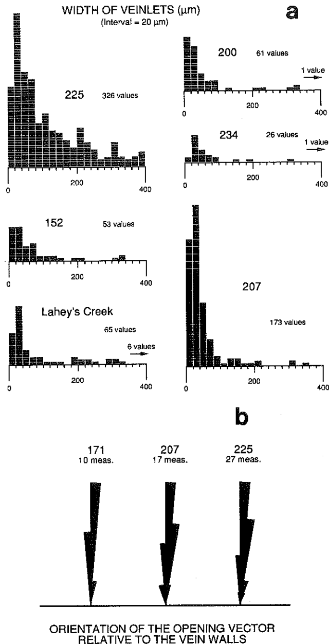
Fig. 8. Geometrical characteristics of quartz veinlets in samples from several deposits. (a) Histograms of veinlet widths. (b) Rose diagrams of the opening directions ( 5^\circ angle classes).
