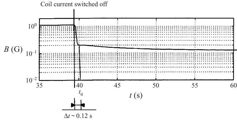
FIGURE 6. Typical time evolution of B_\theta in the vicinity of pump 3. After the current is switched off in the copper coil, the ohmic decay of the electrical current in the coil lasts about 0.12 s.
