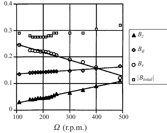
FIGURE 5. The mean field components B_r, B_\theta, B_z (in G) and the modulus of the total field |B_{total}| versus the velocity of pump 2.
