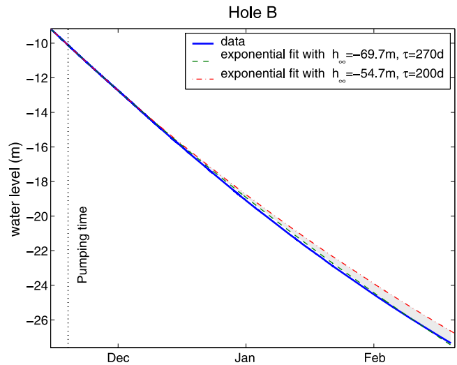
Figure 3. Evolution of the water level in hole B relative to the wellhead. It is compared with the exponential solutions computed with equation (2). We present here the two extreme sets of parameters \tau = 200 \text{ days} , h_{\infty} = -54.7 \text{ m} (top red dot-dashed line) and \tau = 270 \text{ days} , h_{\infty} = -69.7 \text{ m} (bottom green dashed line), that delineate a range of possible fitting exponentials (shaded area). The maximum departure is 70 cm, over a total change of 18 m. The error is thus less than 3.5% over 3 months.
