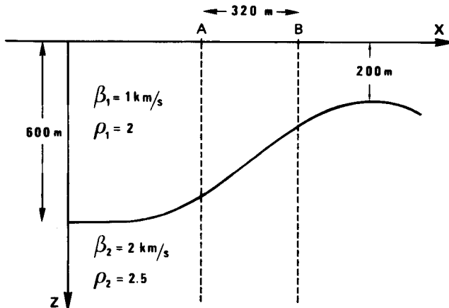
Figure 4. Source-receiver positions and geometry of the medium used to investigate the effect of a dipping interface on a vertical seismic profile (see text).
