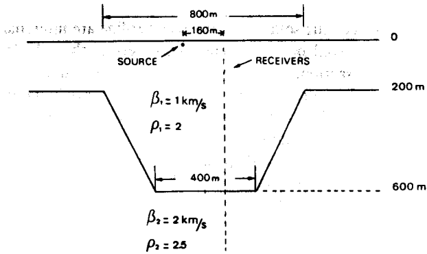
Figure 6. Geometry of the simple model of graben used and synthetic vertical seismic profile.
