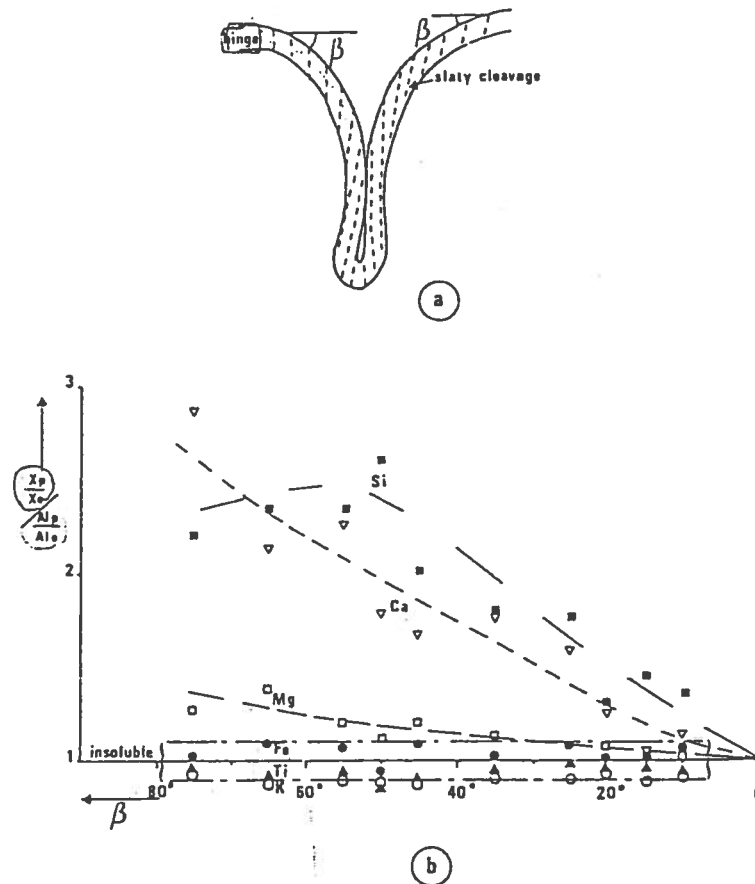
Fig. 2. Mobility test of elements Si, Ca, Mg, Fe, Ti and K (compared with a reference element Al) along a folded layer, as the layer dip ( \beta ) increases. (a) Fold example (Fig. 5). (b) Evolution of the ratio X(p)/X(e) to Al(p)/Al(e) with angle \beta . X(p) and X(e) are the concentrations of an element X in the protected zone (hinge) and in exposed zones (limbs), and Al(p) and Al(e) the respective concentrations of Al. Elements whose ratios vary from 0.9 to 1.1 (variation due to various inaccuracies, see text) without any perceptible evolution as deformation and \beta increase are considered to be contained in insoluble minerals. The calculated \Delta values are given in Fig. 5.
