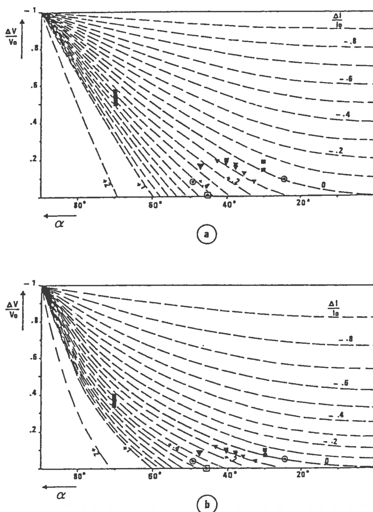
Fig. 7. Relations between \Delta , \Delta l/l_0 and \alpha for the two transfer models defined in Fig. 4. \Delta is the volume change \Delta V/V_0 , \Delta l/l_0 the change in length parallel to the layer in the fold limb and \alpha the angle between hinge and limb. (a) is the open system, and (b) the closed system. The values obtained for various natural examples are plotted on these diagrams and discussed in the text. Each symbol represents one limb-hinge pair. See Fig. 4 for \Delta calculations. Black squares: Jurassic, Col des Saisses, Savoie (also in Figs. 3b and 9a). Black triangles: Jurassic, Col du Lautaret, Hte Alpes (also in Figs. 3c and 9b). Other symbols: Jurassic, west cover of Belledonne, Isere, France.
