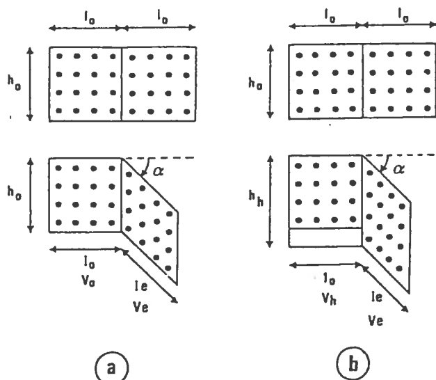
Fig. 4. Material transfer models in the limb-hinge pair of a straight-limbed fold. The limb deformation is simulated by a shear zone with volume change normal to the shear-zone walls, by loss of soluble elements. The quantity of insoluble minerals (black dots) remains constant. Two types of behaviour can be distinguished (see also Fig. 7). (a) The soluble elements leave the limb and the whole limb-hinge pair. This is known as an open system: \Delta V = V_e - V_o ; I_p/I_e = (1 + \Delta) = (1 + \Delta/l_o) \cos \alpha . (b) The soluble elements leave the limb and relocate in the hinge: this is known as a closed system: \Delta V = V_e - V_o = V_h - V_o ; I_p/I_e = (1 + \Delta)/(1 - \Delta) = (1 + \Delta/l_o) \cos \alpha .
