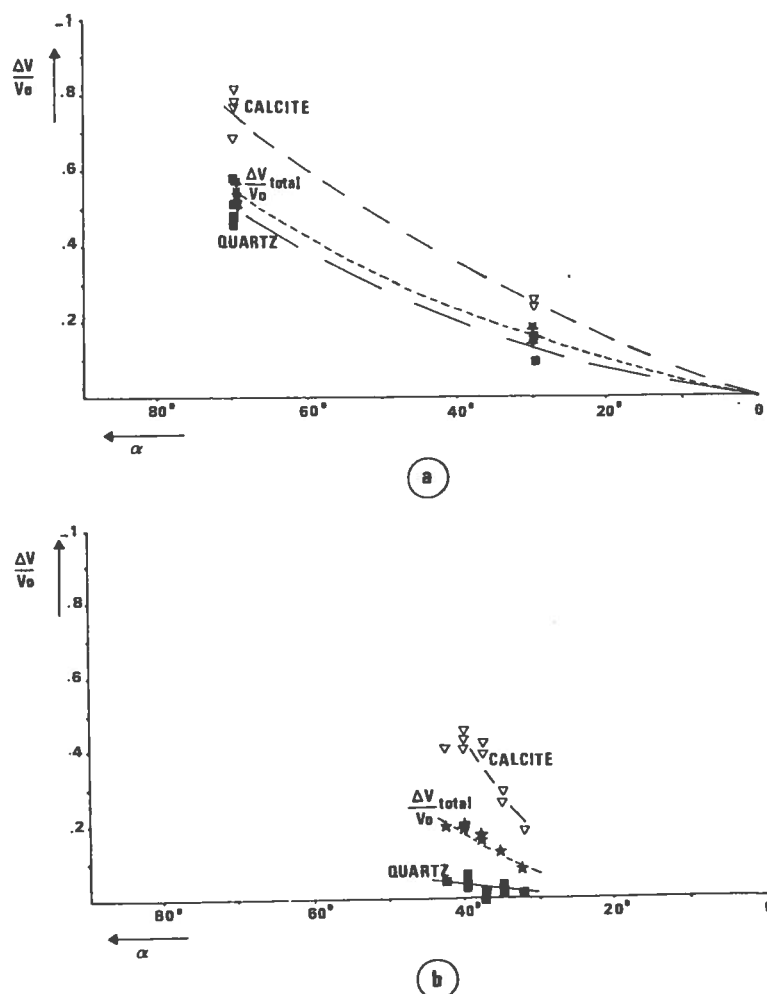
Fig. 9. Comparison of the behaviour of the various soluble minerals by pressure-solution and evolution as deformation increases (increase in limb-hinge angle \alpha ). Same \Delta calculations as in Fig. 8. The folds are those of Figs. 3 and 7; (a) is the black square in Fig. 7 and (b) the black triangles in Fig. 7. Crenulation cleavage is associated with the folds. See Fig. 8 for comparison with fold with slaty cleavage.
