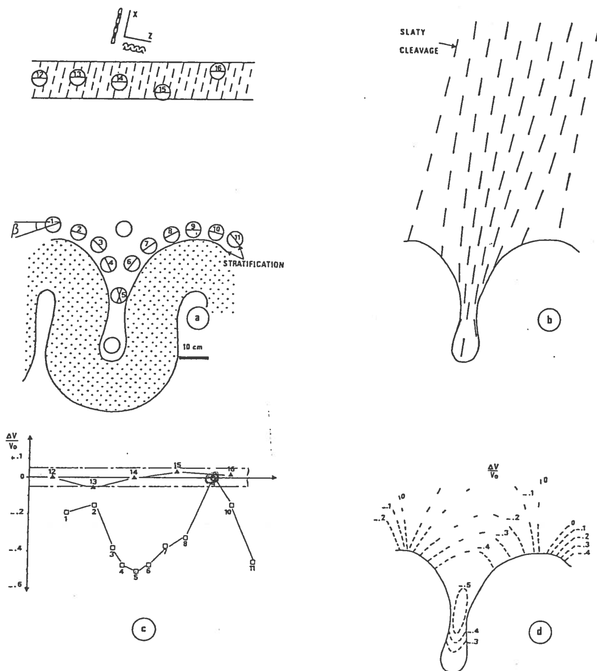
Fig. 5. Estimation of volume-change values and of their relations with finite strain values in the slaty matrix around the buckle fold of a competent layer. (a) Location of core samples, and layer dip ( \beta ) for each sample. The bottom boundary of the studied zone is the competent folded layer, the top boundary is a horizontal layer. Principle strain axes X and Z are shown (b) Dip of slaty cleavage planes on a cross-section normal to the fold axis. (c) Variations in \Delta values (volume change \Delta V/V_0 ) in two layers, along a horizontal axis. Samples no. 14 (top layer) and no. 9 (bottom layer, just above the competent folded layer) are the reference zones for each layer. It will be noted that the two layers have very different behaviours. The chemical composition of the top layer (triangles) is almost homogeneous whereas that of the bottom layer (squares) reveals a substantial chemical differentiation. (d) Distribution of the \Delta values in the slaty matrix, deduced from the previous values and used to calculate the finite strain values in this zone (Fig. 6b).
