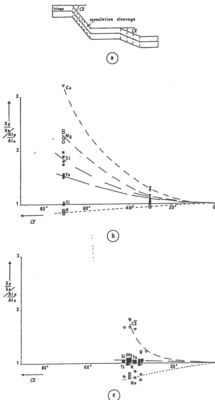
Fig. 3. Mobility test of various elements (compared with a reference element Al) in two limb-hinge pairs of straight-limbed folds, as the limb-hinge angle ( \alpha ) increases. (a) is the fold sketch and (b) and (c) the evolution of the ratio X(p)/X(e) to Al(p)/Al(e) with angle \alpha , as in Fig. 2. Elements whose ratios vary from 0.9 to 1.1 are considered to be contained in insoluble minerals. The \Delta values for each limb-hinge pair of (b) are given in Fig. 7 (black squares), and in Fig. 9(a). The \Delta values for (c) are given in Fig. 7 (black triangles), and in Fig. 9(b). The size of the limb-hinge pair varies from 1 cm to 1 dm.
