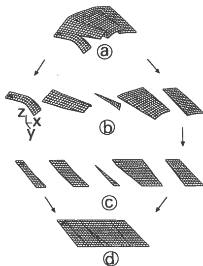
Fig. 1. Sketch of a solution to balance a folded and faulted layer (perspective view). A thin competent layer is restorable to an initial horizontal state if its deformation occurs without change of thickness, and if this layer is well drawn. (a) Deformed state, folded and faulted layer. (b) Partition of this folded and faulted surface into several zones (five) in order to have a single valued mathematical function between the X , Y and Z values of co-ordinates on the surface (after interpolation between spaced data). (c) Unfolding of each zone (limited either by faults or vertical strata) by the computer program. (d) Fitting of these zones to reconstruct the initial (horizontal) state of the layer.
