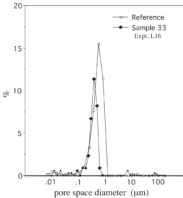
Fig. 8. (a) Cumulative pore diameter distribution curves measured by Hg injection for samples from L16 and an undeformed reference sample. The two samples adjacent to the interface (samples 33, 35) show the largest decrease in porosity and the most significant pore diameter shifts with respect to the reference. (b) Individual normalized porosity % vs. pore space diameters for sample 33 and a reference. These curves show more clearly the overall decrease in porosity of sample 33, as well as a shift in the pore diameter populations, from a median of 0.8 \mu\text{m} for the reference to 0.3 \mu\text{m} for sample 33.
