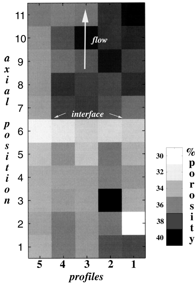
Fig. 9. Gray scale representation of water saturation porosities measured for samples 1-55, L16 (cut-away view along axis- compare to Fig. 7). The maximum measured porosity (40.4%) is indicated in black, the lowest (29.5%) is indicated in white. The overall pattern does not indicate any obvious zones of connected high porosity at the cm-scale. The most obvious feature is a zone of very low porosity (ranging from 30.1-31.1%) immediately adjacent to the interface of the two cores, on the upstream side. The indicated profiles and axial positions refer to Figs. 10 and 11a.
