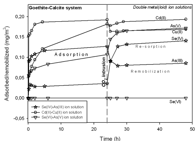
Figure 5. Competitive adsorption/remobilization of binary metal(loid) ions by using goethite-calcite composite as adsorbent. Two ions were arbitrarily combined as follows: As(III)–Se(IV), As(V)–Se(VI), or Cd(II)–Cu(II). A similar initial ion concentration (about 50 mg/L for each element) was used and the adsorbed/remobilized amount was normalized with respect to the initial available surface area (3 g × 90 m 2 /g).
