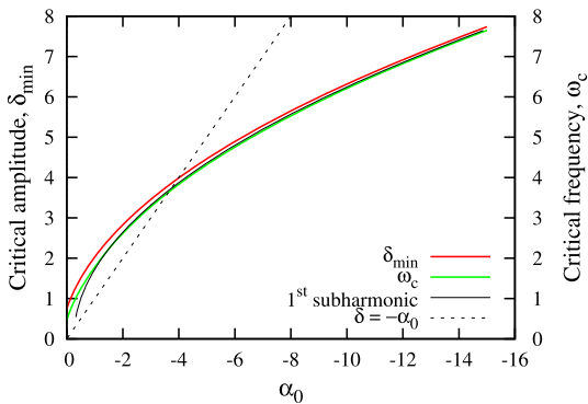
Fig. 4. Minimal oscillation amplitude and critical frequency versus subcritical rotation rate parameter ( \alpha < 0 ).
