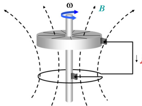
Fig. 1. Sketch of a homopolar disc dynamo.
