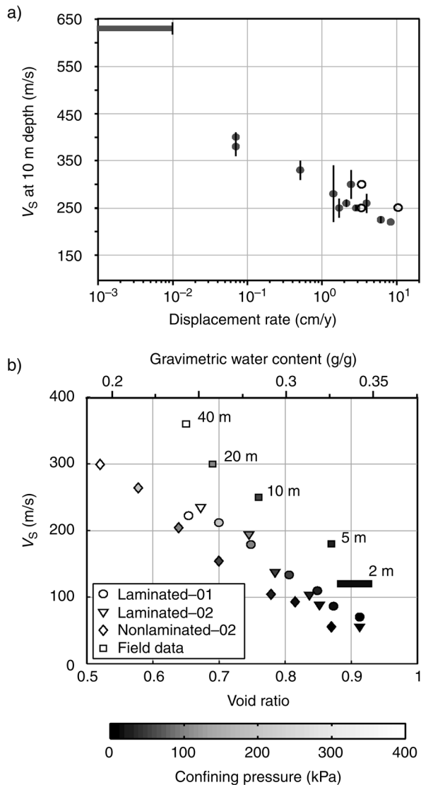
Figure 3. Measured V_S variations. (a) Evolution of shear-wave velocity values (with error bars) as a function of displacement rates, at a depth of 10 m. Data are from surface-wave inversion and SH refraction studies for the profiles shown in Figure 2. The three empty circles correspond to the new measurements. The point outside the landslide ( V_S = 630 m/s) exhibits no measurable displacement and is represented as a thick line with a maximum displacement rate of 0.01 cm/year. (b) Evolution of V_S as a function of void ratio and water content for three saturated samples and field data. The shaded scale indicates the confining pressure. Modified from Bièvre et al. (2010).
