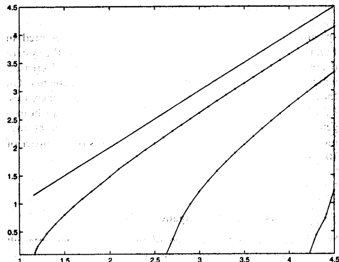
Figure 3. The functions \lambda_0 = \Lambda_0(\beta) , \lambda_1 = \Lambda_1(\beta) , \lambda_2 = \Lambda_2(\beta) and the asymptote \lambda = \beta . Note that positive eigenvalues are reached when \beta > \beta_0 . The static eigenvalues \beta_i can be seen in connection with the dynamic spectral problem. The \beta_i are defined as it follows: \{\beta_i / \Lambda_i(\beta_i) = 0\} .
