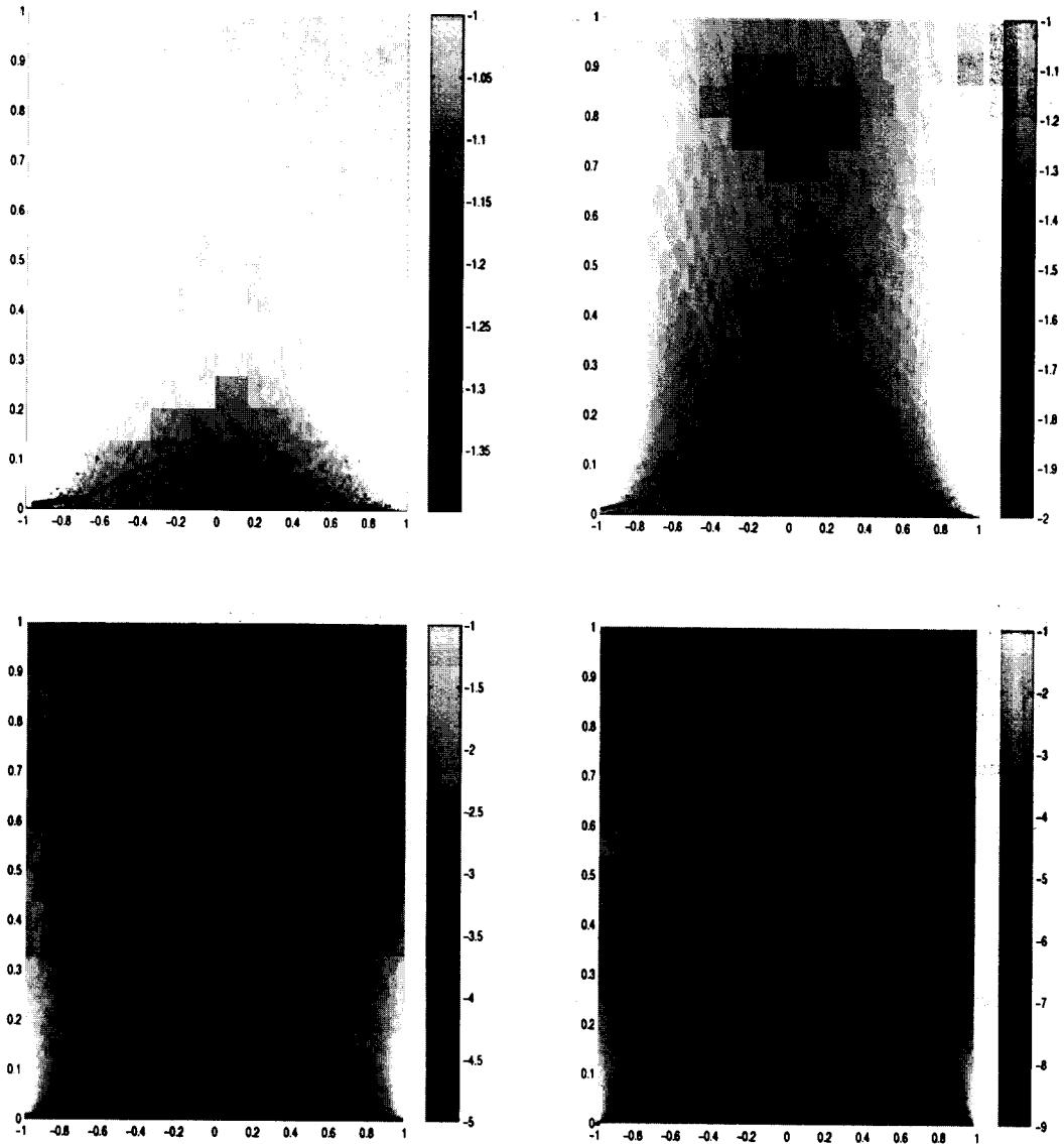
Figure 9. Map view of the B_\beta(x_1, x_2) in the vicinity of the fault for different values of the weakening parameter. From left to right and top to bottom: \beta = 1.2, 1.5, 3, 5 . Note the same shape of the function in the four different cases. The black line emphasizes the limit of the domain of confidence over which the function is nearly constant and equals \beta . The size of this domain is an increasing function of \beta .
