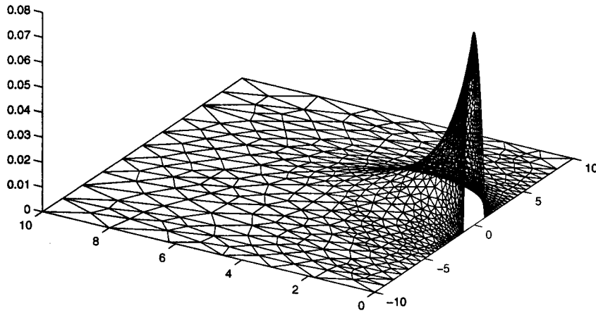
Figure 2. The first nondimensional static eigenfunction \varphi_0(x, y) . The maximum is located at the centre of the fault. The distribution of \varphi_0 on the fault is in good agreement with the slip distribution obtained by FDM. We note the rapid decay of \varphi_0 with x_2 the perpendicular coordinate.
