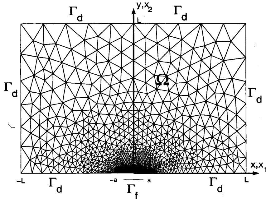
Figure 1. Geometry of the problem. \Gamma_f = [-a, a] is the frictional surface. \Gamma_d is the fictitious boundary. \Omega = [-L, L] \times [0, L] is the elastic half space. x and y are the two coordinates. For symmetry reasons, we consider only y > 0 values. \Omega is meshed with triangular elements using Delaunay conditions. Note the increase in the number of elements near the fault \Gamma_f .
