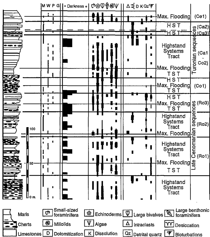
Figure 6. Sedimentological data and interpretation of the upper part of the Arcurquina Formation in the Arcurquina section (Arequipa, southern Peru).
