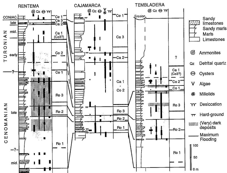
Figure 4. Summarized sedimentological data and interpretation for the late Cenomanian–Turonian sections of northern Peru.
