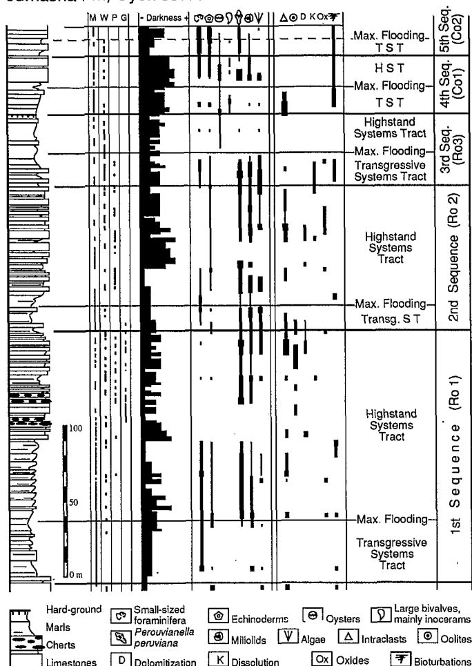
Figure 5. Sedimentological data and interpretation of the upper part of the Jumasha Formation in the Oyón section (central Peru).
