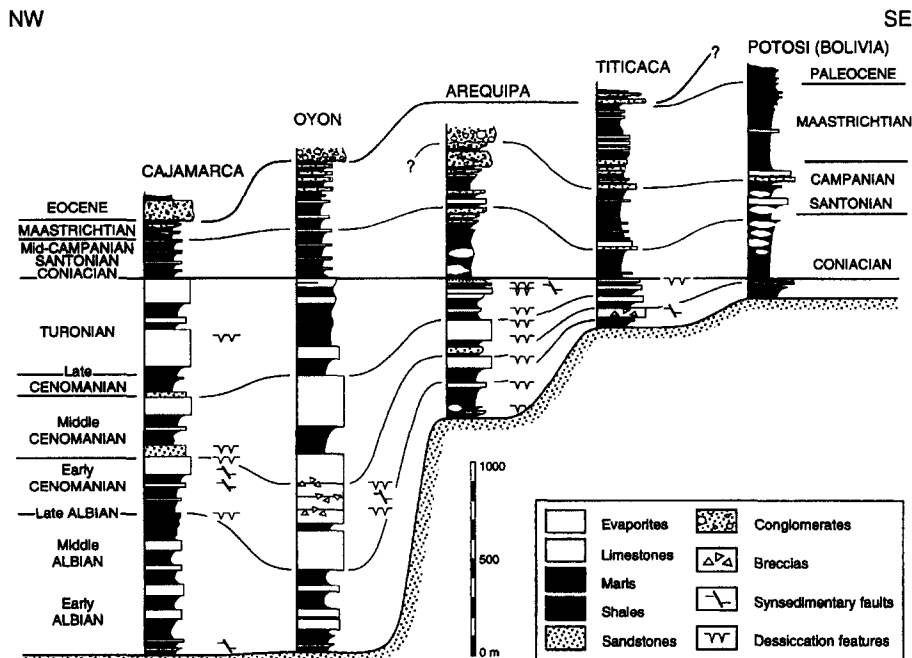
Fig. 3. Representative sections through the Peruvian and Bolivian continental margin, showing the sedimentary evolution between Albian and Eocene times (location on Fig. 1). Data are from Jaillard (1987) for Cajamarca and Oyón, Jaillard (1994) for Arequipa, Jaillard et al. (1993) for Titicaca and Sempéré (1994) for Potosi.
