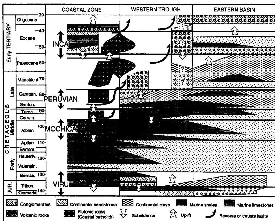
Fig. 2. Sketch of the sedimentary, tectonic and magmatic evolution of the Peruvian margin during Cretaceous and Paleogene times.
