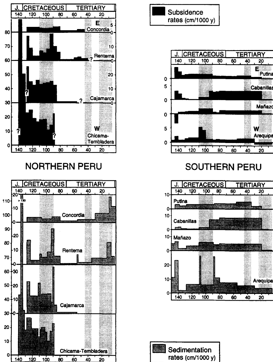
Fig. 4. Decompacted subsidence and sedimentation rates along two profiles across the Peruvian margin (location on Fig. 1).
