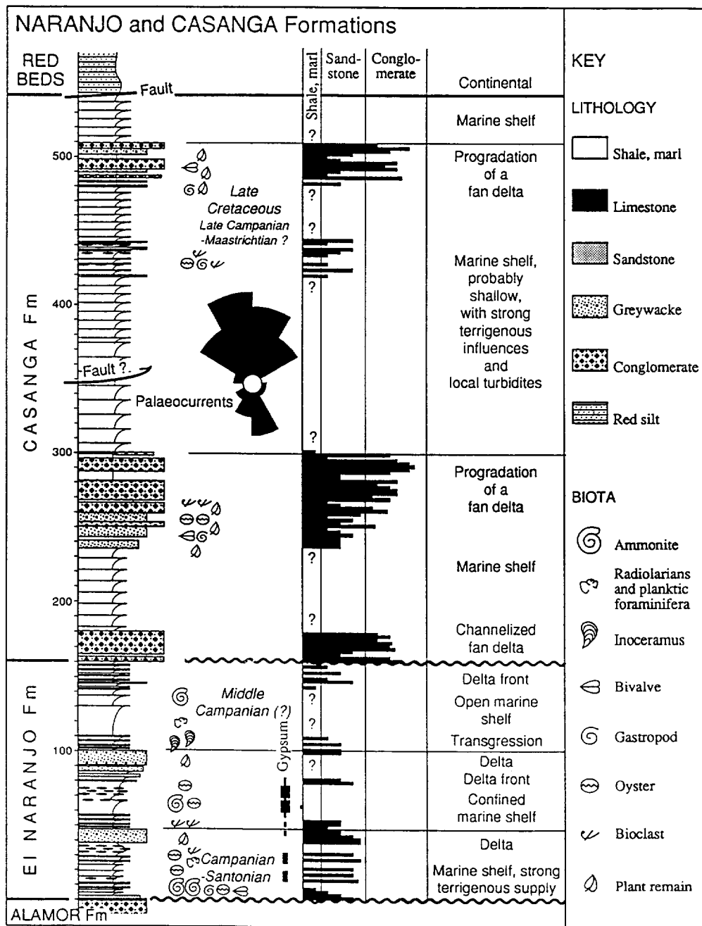
Fig. 4. Section of the Naranjo and Casanga Formations (Santonian-Maastrichtian) of the Río Playas area.
