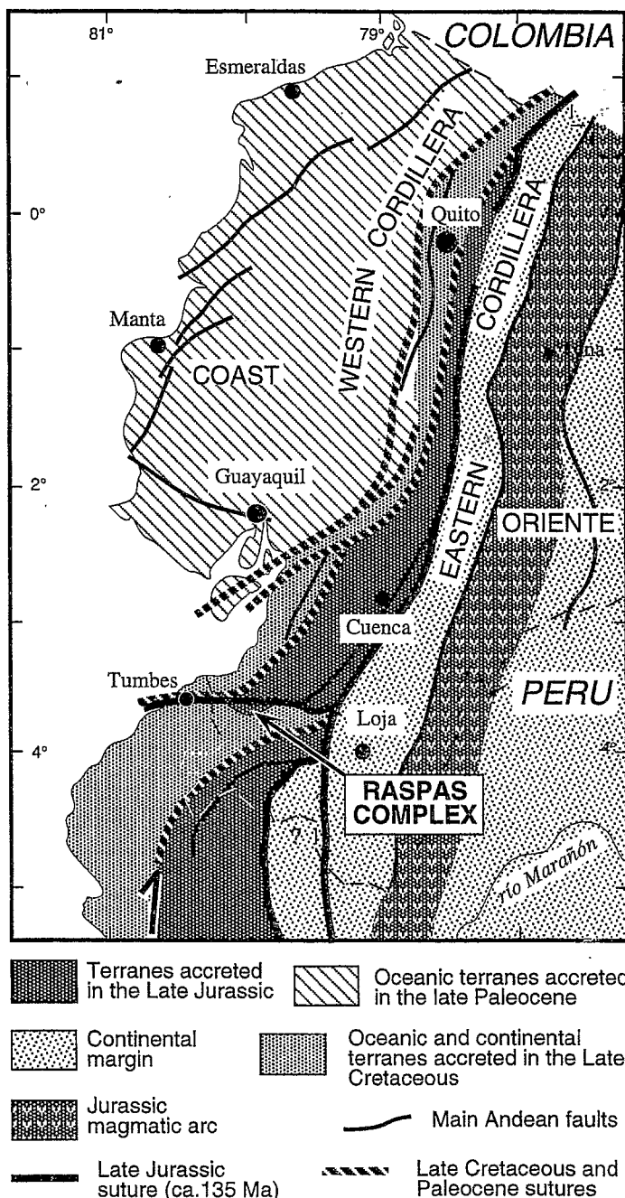
Figure 1. Outline geologic and terrane map of Ecuador, showing location of Raspas metamorphic complex.
