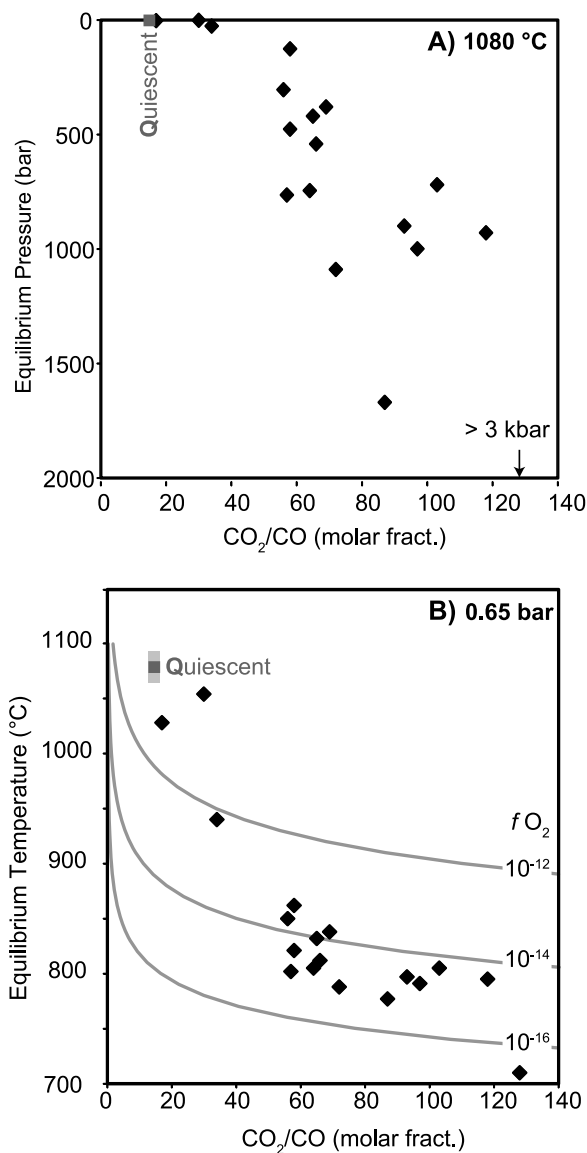
Figure 8. Equilibrium pressures and temperatures of 18 explosions measured in December 2005 as a function of CO 2 /CO. (a) Equilibrium pressures at a constant temperature of 1080°C. This assumes that chemical reactions were slow enough to preserve the gas composition at depth despite slug ascent and decompression. The dark gray point marks the median value for quiescent degassing. Note that one explosion would equilibrate at a pressure higher than the validity limit of the model. (b) Equilibrium temperatures at a constant atmospheric pressure. This assumes that chemical reactions were fast enough to keep pace with ascent-driven decompression. The dark gray point marks the median value for quiescent degassing and the light gray area spans the full range of calculated temperatures. Grey curves mark constant oxygen fugacity values and illustrate how the CO 2 /CO ratio varies with temperature.
