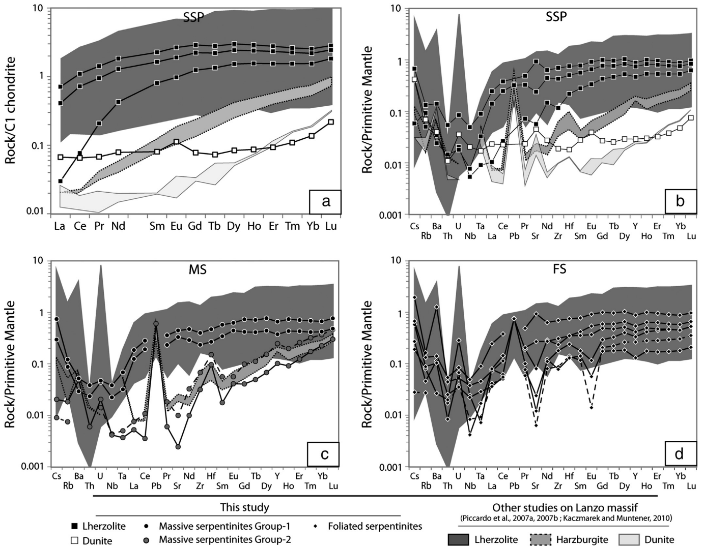
Fig. 5. Whole rock patterns of the different lithologies composing the Lanzo massif. (a) and (b–c–d) patterns are respectively chondrite and primitive mantle normalized; normalizing values are from Sun and McDonough (1989). Symbols are indicated in the figure. Previous analyses of Lanzo peridotites are shown in comparison (shaded areas). (a) Whole rock REE patterns of different type of SSP. (b) Spidergram of SSP. (c) Spidergram of MS. MS analyses do not differ from SSP analysis. Dashed line: LZ26c (massive serpentinite lens embedded by foliated serpentinite). (d) Spidergram of FS. Dashed line: LZ26a (foliated serpentinite embedding LZ26c).
