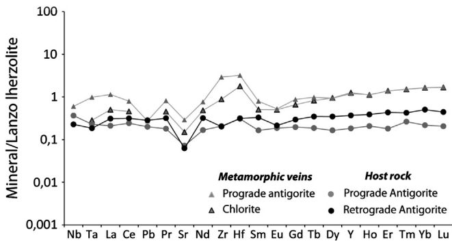
Fig. 11. Mean value of trace elements of the prograde and retrograde antigortites and chlorite of the metamorphic veins and serpentinite host rocks normalized to the composition of the slightly serpentinized lherzolite. The prograde and retrograde antigortites of the host rock do not show fractionations of trace elements relative to the initial protholite composition during the successive serpentinization steps occurring from the ridge to the subduction. The prograde antigortite/chlorite of the metamorphic veins fractionate HREE and HFSE demonstrating a different behaviour during serpentinization processes.
