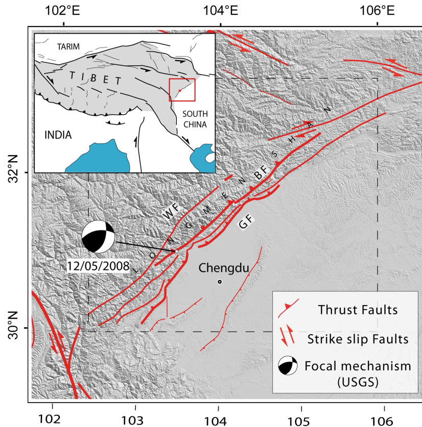
Fig. 1. The study area struck by the Sichuan earthquake. Quaternary active faults and their kinematics are plotted in red (modified from Tapponnier and Molnar, 1977). BF = Beichuan fault; WF = Wenchuan Fault; GF = Guanxian Fault. The dotted rectangle corresponds to the location of Figs. 2 and 3.
