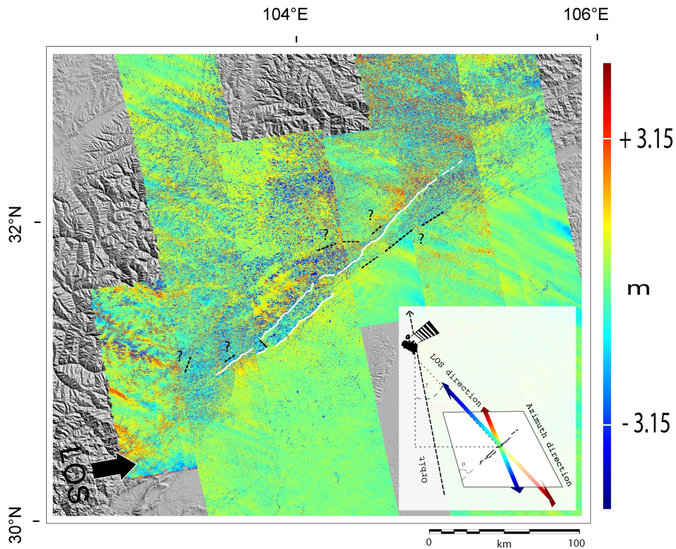
Fig. 3. Offsets in the azimuth direction (azimuth streaks reduced). Our interpretation of the rupture is plotted in white. Dark dashed lines represent possible rupture segments not yet observed in the field. The inset represents the PALSAR acquisition geometry relative to our case study. Colour scaled arrows indicate the slant range and azimuth direction of the measured offset relative to the rupture position. This is a key to interpret the sense of displacement in Figs. 2 and 3. \gamma = sight angle ( 34^\circ ), \theta = angle between the rupture strike and azimuth direction ( \sim 65^\circ ).
