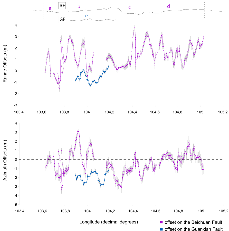
Fig. 4. Plot of range and azimuth offsets measured along the strike of the Beishuan fault (BF) and Guanxian Fault (GF) ruptures (plotted on top as reference). Major components of slip are dextral or reverse when offsets are positive and negative, respectively (see text for details). Longitude values are sampled along the strike of the rupture.
