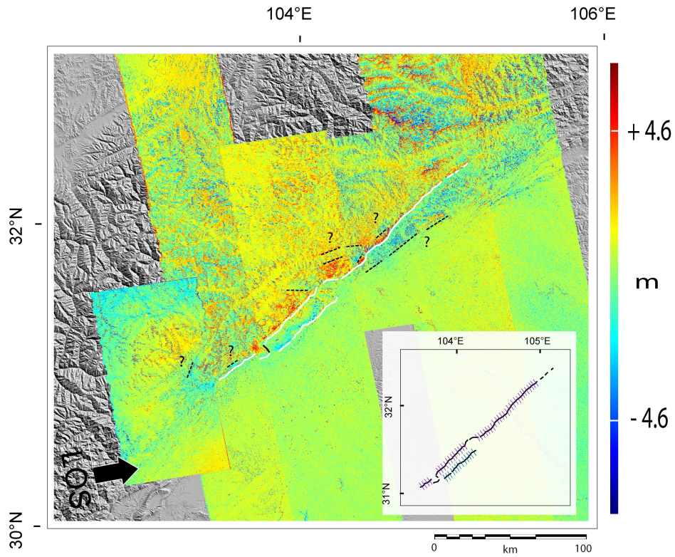
Fig. 2. Offsets in the range direction. Our interpretation of the rupture is plotted in white. Dark dashed lines represent possible rupture segments not yet observed in the field. The \sim 10 km rupture segment striking NW-SE (perpendicular to BF and GF ruptures) is presented in bold black (here and in Fig. 3). The inset represents the average location of profiles used in the stack to retrieve the offset plots in Fig. 4. See the inset of Fig. 3 for the satellite acquisition geometry.
