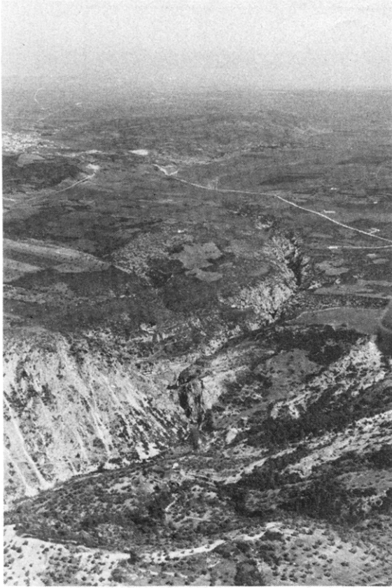
Fig. 8. View looking eastwards up the Livadostros valley towards Platea. Note the undulating erosion surface cut into by the river gorge and the lineation on the right, which is also visible in Fig. 11. The eastern section of the March 4 fault break follows the contact between the limestone and the erosion surface alluvium on the left before crossing the gorge.
