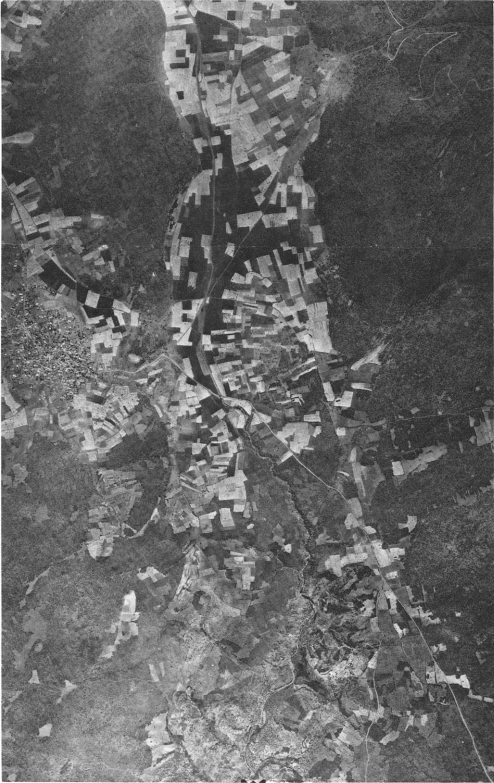
Fig. 11. Air photo of the Livadostros valley (see Fig. 6 for location). The 1981 fault breaks follow the limestone-alluvium contact in the eastern (right) part of the picture, and cross the valley at the dissected topography where the gorge starts to widen.
