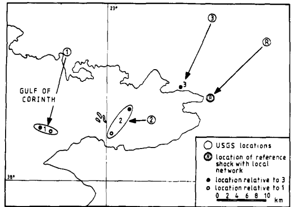
Fig. 13. Epicentre locations. Arrows show the difference between U.S.G.S. and relocated epicentres for the shocks of February 24 (1), February 25 (2), March 4 (3) and March 7 (R).
