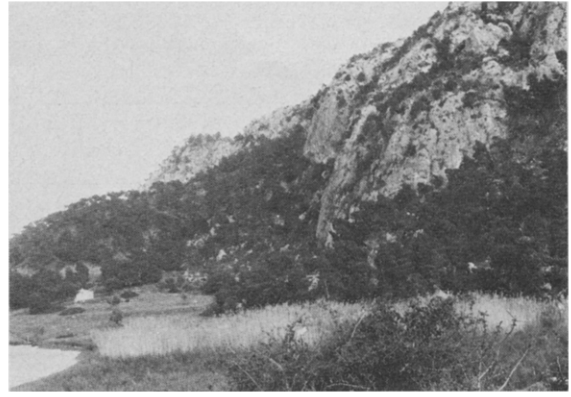
Fig. 19. A sinking region 2 km east of Skinos, showing a swampy, inundated coastline, behind which is the limestone cliff of the lower of the two major southern escarpments.
