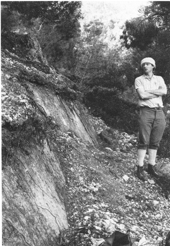
Fig. 4. The southern fault break 2 km east of Pision. A typical outcrop of the fault face against unconsolidated angular scree.
