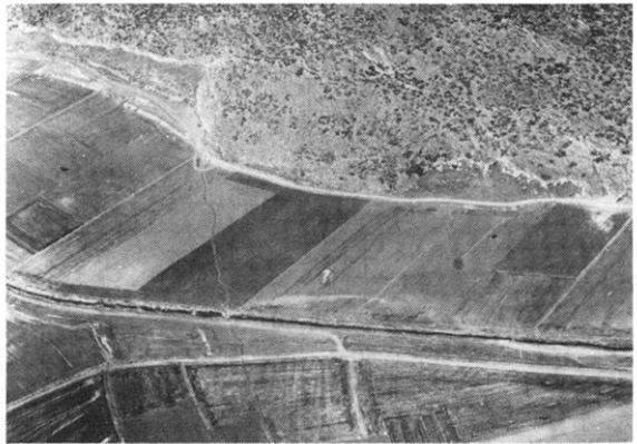
Fig. 10. The eastern end of the March 4 fault break, where it leaves the limestone scarp, which continues eastwards, and crosses the valley towards Platea. View looking NW.
