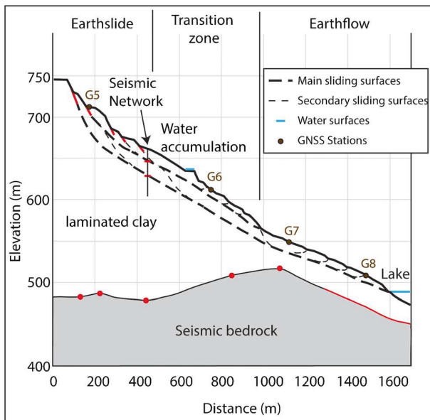
Fig. 9 Interpretative cross section of the Harmalière landslide from the topography extracted from the LiDAR DEM acquired in November 2019. Red dots: bedrock roof from H/V measurements refined from Bièvre et al. (2011) results. Red part of the bedrock corresponds to the 1950 topography. Red bars: constraints on the scarps and shear surface deduced from the seismic network
