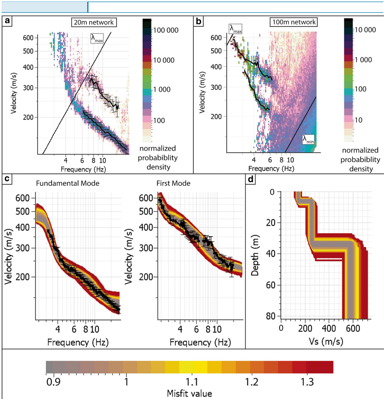
Fig. 5 Seismic noise analysis using the two arrays. a Dispersion histogram of the 20 m array and picked curves with error bars (black). b Dispersion histogram of the 100 m array and picked curves with error bars (black). c Rayleigh wave dispersion curves (black dots with error bars) picked for the fundamental mode (left) and the first higher mode (right) from the dispersion map. d Inverted vertical Vs profiles using the neighborhood algorithm (Wathelet 2008). Corresponding misfit values are indicated by colors on model results (Fig. 5d) and dispersion curves (Fig. 5c)
