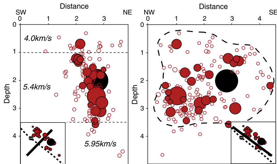
Fig. 2. The Vuache strike-slip fault: section through the aftershock zone, on the left a SW–NE section (with the velocity model), on the right a NW–SE section, black solid circle = main shock, red solid circles = aftershocks of magnitude 1 and more, open red circles = aftershock of magnitude less than 1. The thick dashed line is the inferred extension of the rupture area. Insets (map view) give the location of the cross-section (solid black line) relative to the geological trace of the fault at the surface (dotted line). Adapted from Thouvenot et al. (1998).
