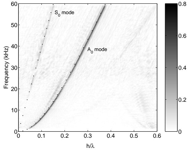
FIG. 3. f-k transform of the source-receiver impulse responses. X-axis: dimensionless wavenumber ( h is the slab thickness). Dots are theoretical solutions of Eq. 1.
