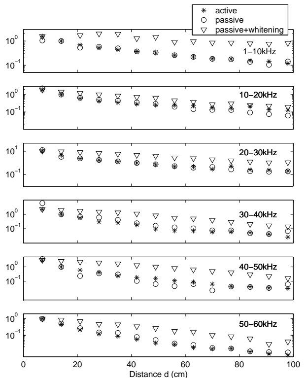
FIG. 7. Amplitude decay obtained in an active experiment (stars) and by correlation (circles) without additional processing, and with whitening (triangles). Attenuation includes geometrical spreading and absorption.
