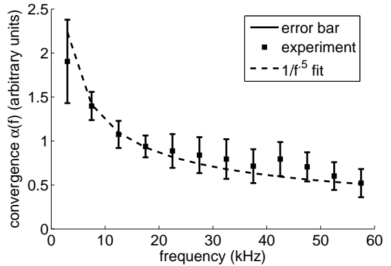
FIG. 10. The fit coefficient \alpha of the SNR is plotted versus the central frequency f of the records.
