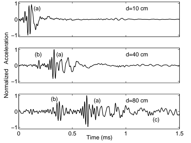
FIG. 2. Source-receiver impulse response h_d(t) for different distances d . (a) Dispersive anti-symmetric A_0 mode propagating at velocities approximately ranging from 150 to 900 m/s. (b) Non-dispersive S_0 mode propagating at \approx 2400 m/s. (c) Reflexions from surrounding edges.
