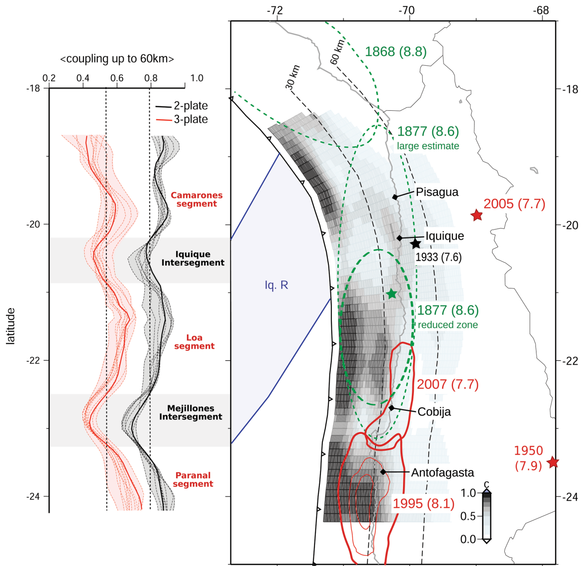
Figure 5. Left-hand side: average coupling coefficient ( \Phi ), versus latitude. ( \Phi is the integration from 0 to 60 km depth of the coupling distribution on the interface, using a 0.2^\circ sliding window in latitude. Greyish curves are for the 2-plate model, redish curves are for the 3-plate model. Solid curves depict the preferred (best-fit) model, and dashed curves depict a subset of alternative models with reasonably good nrms ( <3 for 2-plate models, and <1.5 for 3-plate models). Grey and pink shaded areas depict the envelope of these alternative models and represent the uncertainty of our preferred coupling distributions. Black dotted lines mark the mean value of coupling for each case. Segments ( \langle\Phi\rangle larger than the mean value) and intersegment zones ( \langle\Phi\rangle lower than the mean value) are named on the right-hand side of the graph. Right-hand side: coupling distribution is colour coded and superimposed with estimates of the rupture zones of major instrumental or historical earthquakes (solid red or green dotted ellipses, respectively). Thin red ellipses: 2 m slip contours of 1995 Antofagasta earthquake (Chlieh et al. 2004). Bold green dashed ellipse is the reduced rupture zone we propose for the 1877 earthquake based on (Kausel 1986). Green star: epicentre of the 1877 earthquake (Comte 1991). Black star: epicentre of the 1933, M_w 7.5 Iquique earthquake (Centennial catalogue). Dark blue solid line: rough contours of the Iquique Ridge.
