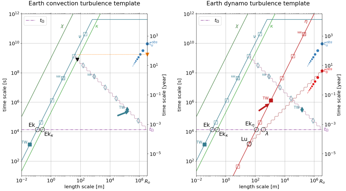
(a) Template for Earth's core rotating convection.
