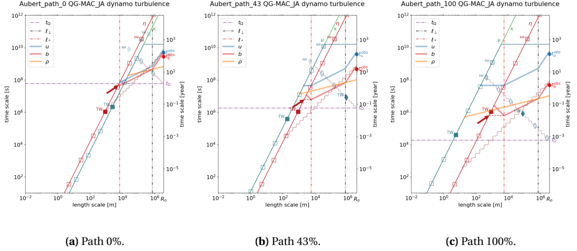
Figure 7. \tau - \ell regime diagrams illustrating the ‘path strategy’ devised by Aubert and colleagues. (a) 0% of path ( \epsilon = 1 ). (b) 43% of path ( \epsilon = 10^{-3} ). (c) 100% of path ( \epsilon = 10^{-7} ). See text for explanations.
