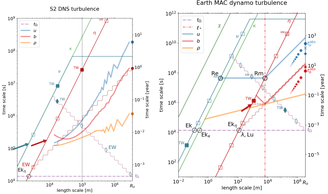
(a) S2 DNS of Schaeffer et al. [2017].
