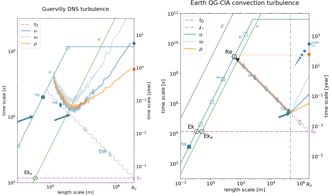
(a) 3D simulation from Guervilly et al. [2019].
