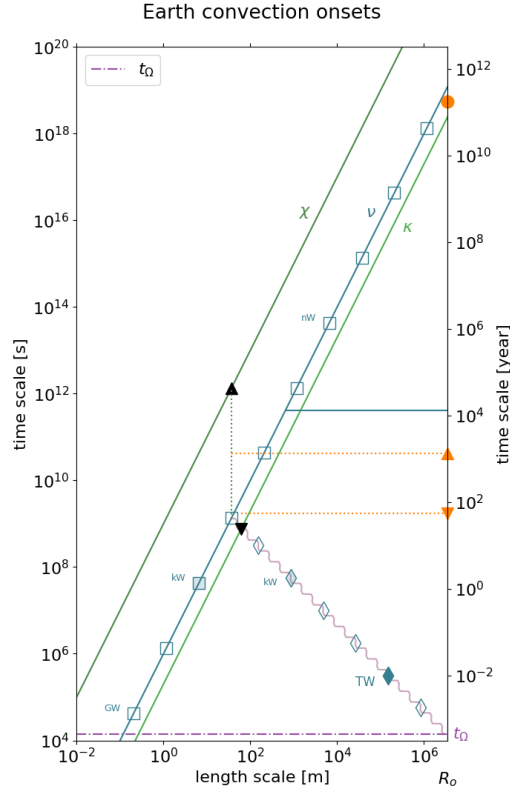
Figure 8. \tau - \ell diagram illustrating convection onset in the Earth's core in the absence of a magnetic field. In the absence of rotation, convection sets in with a cell size comparable with R_o . Orange disk marks the value of \tau_\rho at convection onset. It is half-way between \tau_\kappa(R_o) and \tau_\nu(R_o) , where \text{Ra}(R_o) \sim 1 . Rotation controls the length-scale at which convection sets in. We compare a \text{Pr} < 1 case with a \text{Pr} > 1 case. Black down-triangle marks column radius \ell_c and period \tau_c of the quasi-geostrophic vortices that form at convection onset when considering viscosity and thermal diffusivity ( \text{Pr} < 1 ). Orange down-triangle at \ell = R_o indicates the value of \tau_\rho at onset. Up-triangles display the same quantities when considering viscosity and compositional diffusivity \chi ( \text{Pr} > 1 ). Dotted lines help reading their graphical construction.
