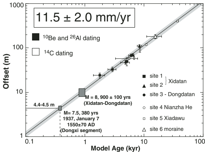
Figure 7. Summary of late Pleistocene–Holocene sinistral slip rates deduced from cosmogenic ^{10}\text{Be} – ^{26}\text{Al} and ^{14}\text{C} dating of alluvial terraces at six sites along the Kunlun fault. Consistency between independent values obtained with different dating techniques implies uniform average slip rate of 11.5 \pm 2.0 mm/yr along 600 km of fault (Van der Woerd et al., 1998, 2000, 2002b).
