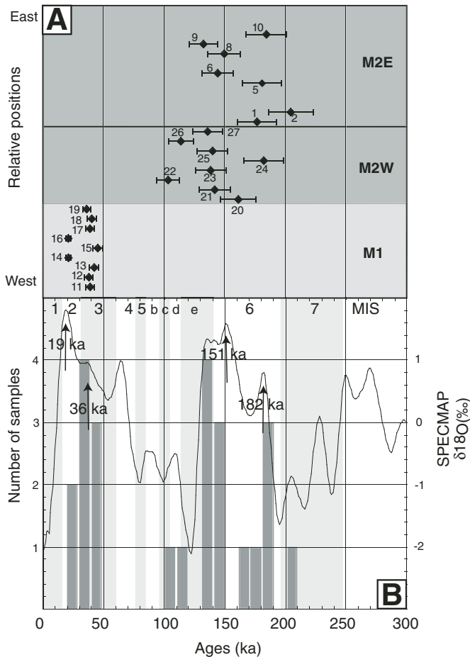
Figure 16. Manikala ages plus SPECMAP. A: ^{10}\text{Be} exposure ages of blocks sampled along M1 and M2 moraine crests. B: Comparison of age distribution (10 k.y. bins) with SPECMAP \delta^{18}\text{O} proxy climate curve ( \delta^{18}\text{O} increases during glacial advances as ^{16}\text{O} is preferentially sequestered in the polar ice caps) shows a simple correlation of main moraine emplacement periods with coldest epochs of marine isotope stage MIS 6, MIS 3, and MIS 2 (LGM).
