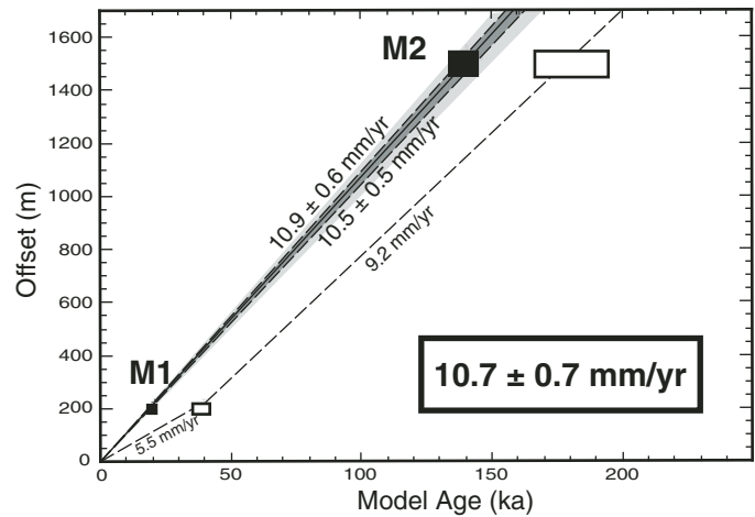
Figure 17. Rates obtained from the offset age relationships for the Manikala moraine complex (Chevalier et al., 2005a). An average rate of 10.7 \pm 0.7 mm/yr is obtained from linking the 1520 \pm 50 m and 220 \pm 10 m offsets with the end of MIS 6 (ca. 140 ka) and MIS 2 (ca. 20 ka), respectively. This association yields a constant slip rate over the entire observation interval. A slip rate of 5.5 mm/yr is implied if the 220 \pm 10 m is linked with the 40 \pm 3 ka age of the older subgroup on M1. This low slip rate over the last ~40 k.y. requires a rate of 9.2 mm/yr between ca. 40 ka and ca. 180 ka to reconcile the rate obtained if the 1520 \pm 50 m offset is linked with the 181 \pm 14 ka age cluster on M2E.
