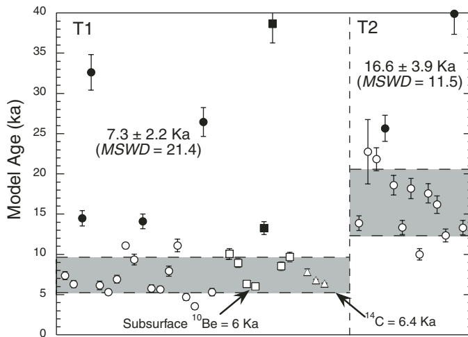
Figure 11. ^{10}\text{Be} exposure model age determinations at Cherchen He (Mériaux et al., 2004). The average values are simple unweighted means with errors equal to one standard deviation for surface samples. The 1\sigma brackets on the average ages are shown as the shaded regions on the figure. ^{10}\text{Be} ages of samples included in the average are shown as open symbols; filled symbols are for ages that were considered as outliers. Surface samples are shown as open and filled circles, and depth-corrected ages of subsurface samples are shown as open and filled squares. Radiocarbon ages are shown as open triangles. Surface samples yield an average age of 7.3 \pm 2.2 ka for T1 and an average of 16.6 \pm 3.9 ka for T2. Sample TU3-71, 71.8 \pm 4.6 ka, has not been plotted in order to improve the resolution in the age range of interest.
