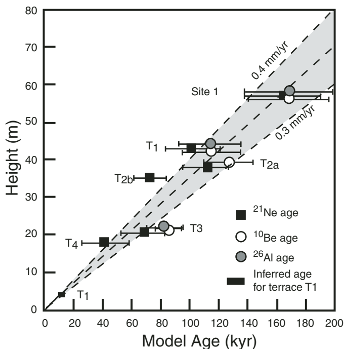
Figure 19. Plot of height above baseline versus model ages of the different terraces. Error bars indicate 2\sigma values (Hetzel et al., 2002). Three dashed lines indicate constant rates of river incision and tectonic uplift of 0.3, 0.35, and 0.4 mm/yr.
