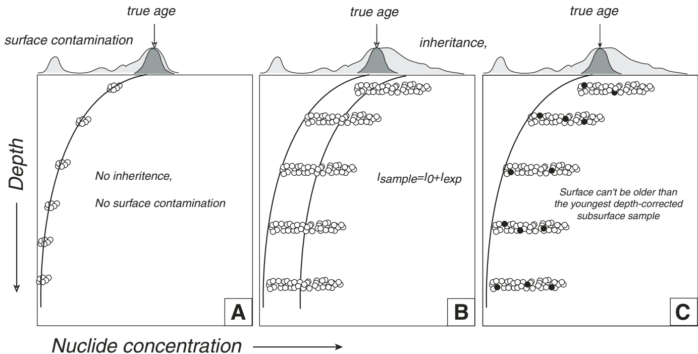
Figure 5. Relationship of surface and subsurface cosmogenic isotope compositions. (A) Surface age frequency distribution in which the “abandonment age” (dark gray) has been mixed with a younger population introduced by surface contamination, but contains no inherited component. Subsurface samples are free of surface contamination, and as there is no inheritance, follow an exponential decrease with depth, reaching zero concentration at the shielding depth. (B) Surface age frequency distribution in which the “abandonment age” (dark gray) has been mixed with a younger population introduced by surface contamination, and an older population associated with inheritance. Subsurface samples are surface contamination-free, but inherited component varies from sample to sample. Amalgamation of multiple samples allows the average inheritance, I_0 , and average exposure concentrations, I_{exp} , to be determined (Anderson et al., 1996; Hancock et al., 1999; Perg et al., 2002; Repka et al., 1997). (C) Similar to B, but with sampling of individual cobbles (filled symbols) instead of amalgamated samples. Since subsurface samples can only be perturbed by inheritance, a limiting isochron can be established, providing a maximum age for the surface (Mériaux et al., 2004).
