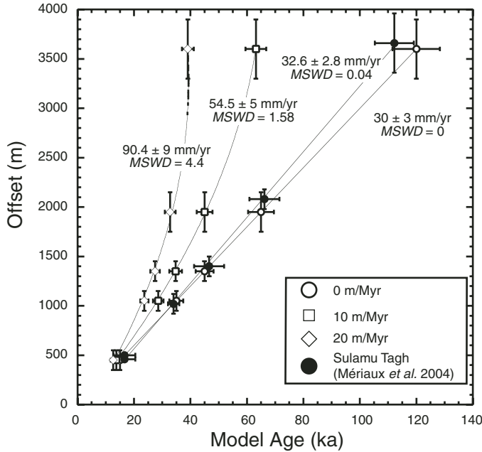
Figure 21. Effects of erosion rate on the apparent slip rate for a fault with a constant slip rate over time. For a fixed set of offset measurements, we assume a slip rate of 30 mm/yr with offsets, ages, and errors similar to those observed at Sulamu Tagh (Mériaux et al., 2004). For the 10 and 20 m/m.y. erosion rate models, we assume that the age is the same as in the zero erosion rate model, but recalculate the nuclide abundance for the different erosion rates. A “zero erosion rate model age” is then derived from these “erosionally decreased” nuclide concentrations. The zero erosion rate model ages generated for different erosion rates are then plotted against the observed offsets. The effect of erosion in decreasing the model ages is most apparent for the oldest samples, and as erosion rate increases, the slip-rate plots depart from linearity and the apparent slip rate increases dramatically. MSWD—mean square of weighted deviation.
