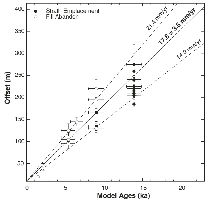
Figure 13. Aksay offset versus model age. Slip rate estimates are derived from using the age of the overlying surface for fill terraces and channels and the emplacement age of the underlying surface for strath terraces, yielding an average Holocene rate of 17.8 \pm 3.6 mm/yr (after Mériaux et al., 2005).
