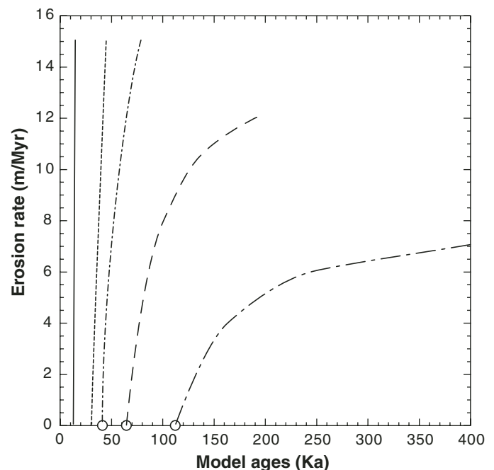
Figure 20. Effects of erosion on model ages. The zero erosion rate model ages for samples with ^{10}\text{Be} concentrations similar to those from the Sulamu Tagh site along the central Altyn Tagh fault (Mériaux et al., 2004) are shown along the abscissa. The curves indicate the true exposure age of a sample with these model ages for different erosion rates. Samples with model ages younger than ca. 60 ka are not significantly affected by erosion, but model ages for older samples can be significantly perturbed.
