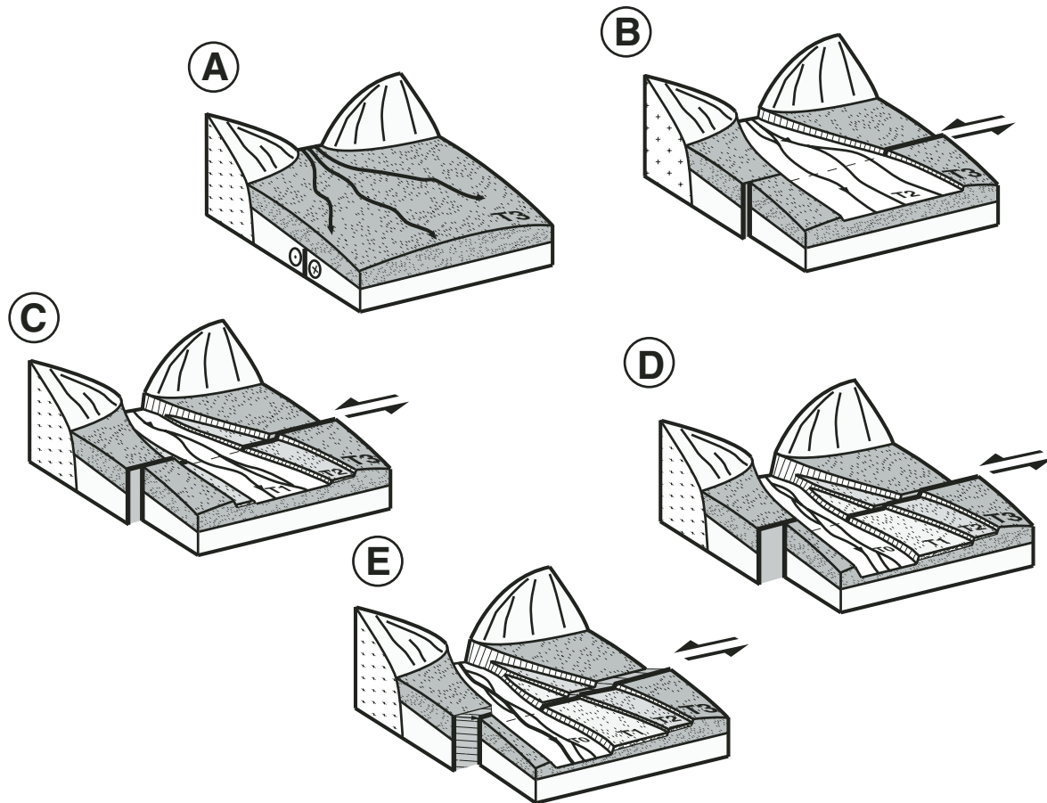
Figure 2. Sequential development of offset terraces associated with strike-slip movement along an active fault. Block diagrams showing plausible sequence of terrace emplacement and stream entrenchment disrupted by strike-slip faulting across bajada in range-front piedmont basin. (A) Emplacement of large fan T3 (fill) at time of large sedimentary discharge. Fault trace is buried. (B) After period of energetic discharge, stream incises channel T2. T3 surface is abandoned and begins to record faulting, but the riser is constantly refreshed by lateral cutting. (C) During new episode of entrenchment, T2 (strath) is abandoned and riser T3/T2, now passive marker, begins to record lateral displacement. Age of T2 abandonment dates riser offset. (D) Successive episodes of terrace beveling and entrenchment of stream due to climatic variation and stream profile evolution lead to formation of several terraces whose risers are offset differently. All episodes may not be recorded by all rivers, and older terraces can be eroded by further incision (see right bank of stream, for example). (E) Similar situation with small vertical slip component. Vertical offset accumulates when terrace is abandoned by stream. Hence, vertical offset of T1 (or T2) is correlated to horizontal T2/T1 (or T3/T2) riser offset, and correlated offsets have ages of T1, or T2, respectively.
