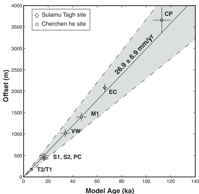
Figure 9. Slip-rate summary on the central Altyn Tagh fault during the last glacial cycle (Mériaux et al., 2004). Open symbols are the preferred slip-rate estimates yielding a bracket of 25–35 mm/yr; the lower bound is largely controlled by the Cherchen He data. The linear regression of the nine data points that determine the upper slip-rate estimates yields a rate of 26.9 \pm 6.9 mm/yr.
