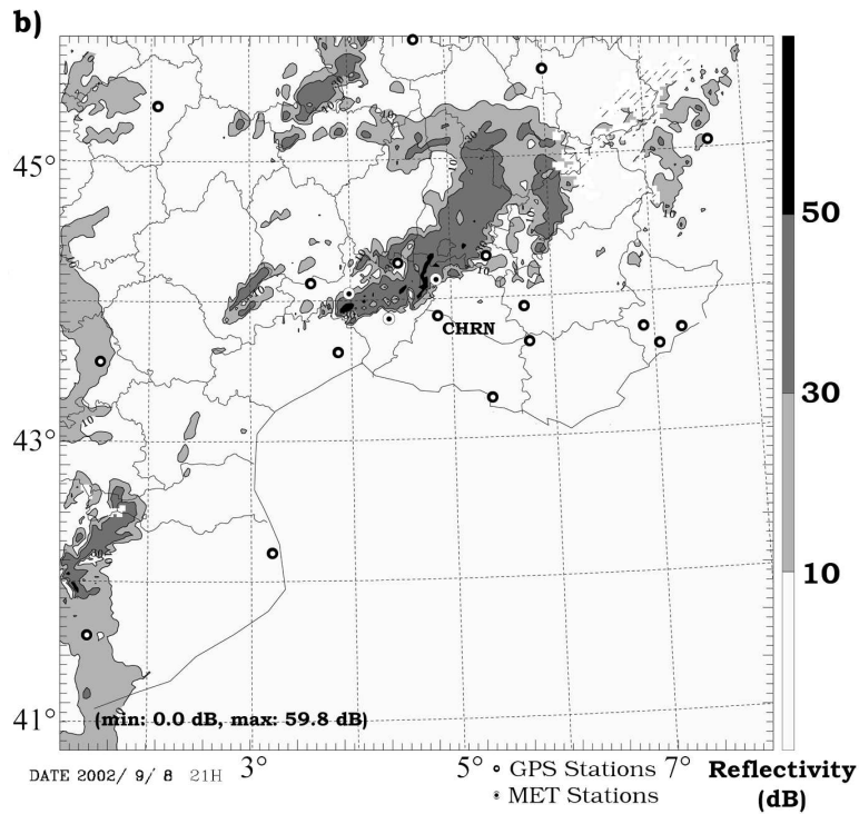
FIG. 2.7 – a) Zenith Hydrometeor Delay (ZHmD in mm) evaluated at 21 UTC on the 8 th September 2002 for the AMA12 experiment. b) Synthetic RADAR reflectivity evaluated for the same experiment at the same time.
