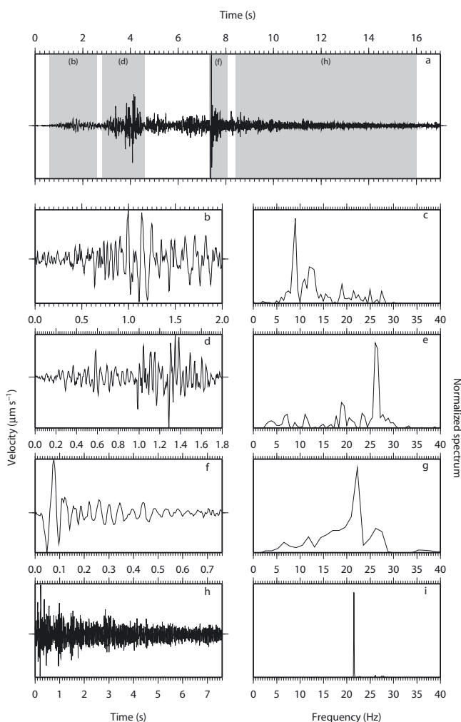
Fig. 3. Velocity seismograms of a type II event recorded at channel 1, and the corresponding power density spectra. The top window (a) shows the entire serac fall signal, lasting for more than 15 s. Boxes marked (b), (d), (f) and (h) are sub-events, shown in more detail in respective windows with corresponding spectra (c, e, g, i) on their right.
