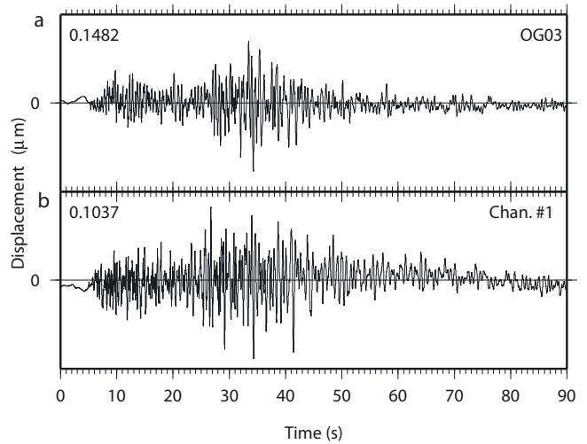
Fig. 13. Vertical displacement generated by a tectonic earthquake recorded at (a) SISMALP station OG03 and at (b) sensor 1. The maximum of displacement is indicated at the top left corner of each window in \mu\text{m} . For sensor 1, we computed an amplification factor of 0.698 which is almost equal to the amplification factor of OG03, 0.700.
