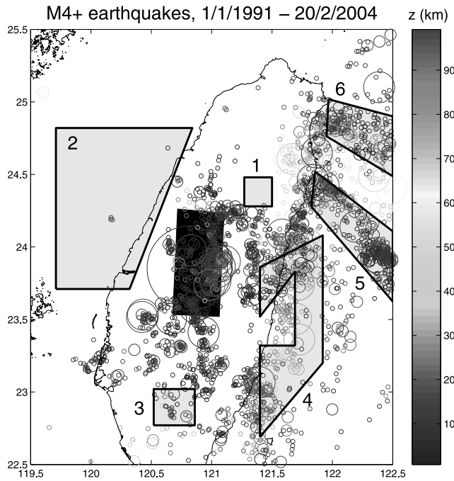
Figure 5. M_{4+} earthquakes in Taiwan, 1991–2004. The Chelungpu fault that ruptured during the Chi-Chi earthquake is sketched by its projection onto the surface, in black. The four areas reported by Ma et al. [2005] to have experienced delayed quiescences plus the two additional zones discussed in section 4.5 are shown in gray: (1) Nansan, (2) Taichung, (3) Kaoping, (4) Huathung, (5) Nanao forearc, (6) Okinawa Trough.
