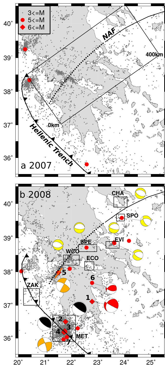
Figure 2. Seismicity in (a) 2007 and (b) 2008 (from the Observatory of Athens catalog) and mechanisms of the events discussed [Zahradnik et al. , 2008; Roumelioti et al. , 2009; www.geophysics.geol.uoa.gr] (red = intra-slab rupture at intermediate-depth; black = subduction earthquakes; orange = strike-slip earthquakes; yellow = extensional earthquakes). The rectangle in Figure 2a outlines the region in supporting information Figure S1. Boxes in Figure 2b show the areas considered in Figure 3a and supporting information Figure S7: MET: Methoni, ZAK: Zakynthos, WCO: West Corinth, ECO: East Corinth, SPE: Sperchios, EVI: Evia, SPO: Sporades, CHA: Chalkidiki. The orange line is the Achaia rupture. Numbers show the chronology of the Peloponnese earthquakes.
