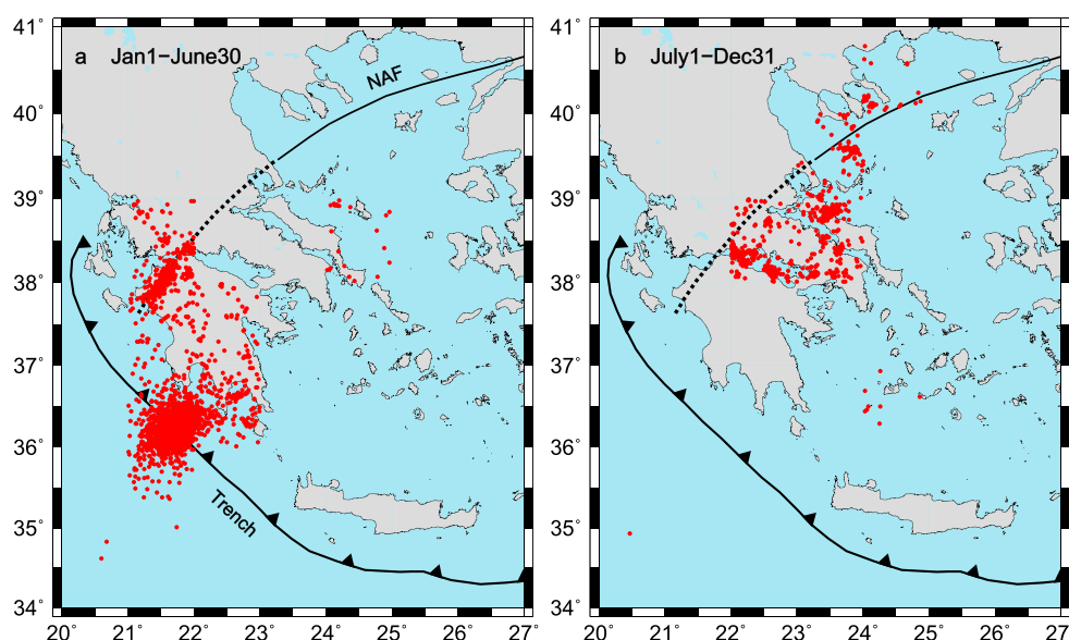
Figure 4. Spread of the deformation in Greece following the slab breakup. (a) Seismicity in the first half of 2008 in areas where the cumulated seismic moment during this period is more than 10 times its corresponding value of previous years (2003–2007). (b) Same as Figure 4a for the second half of 2008.
