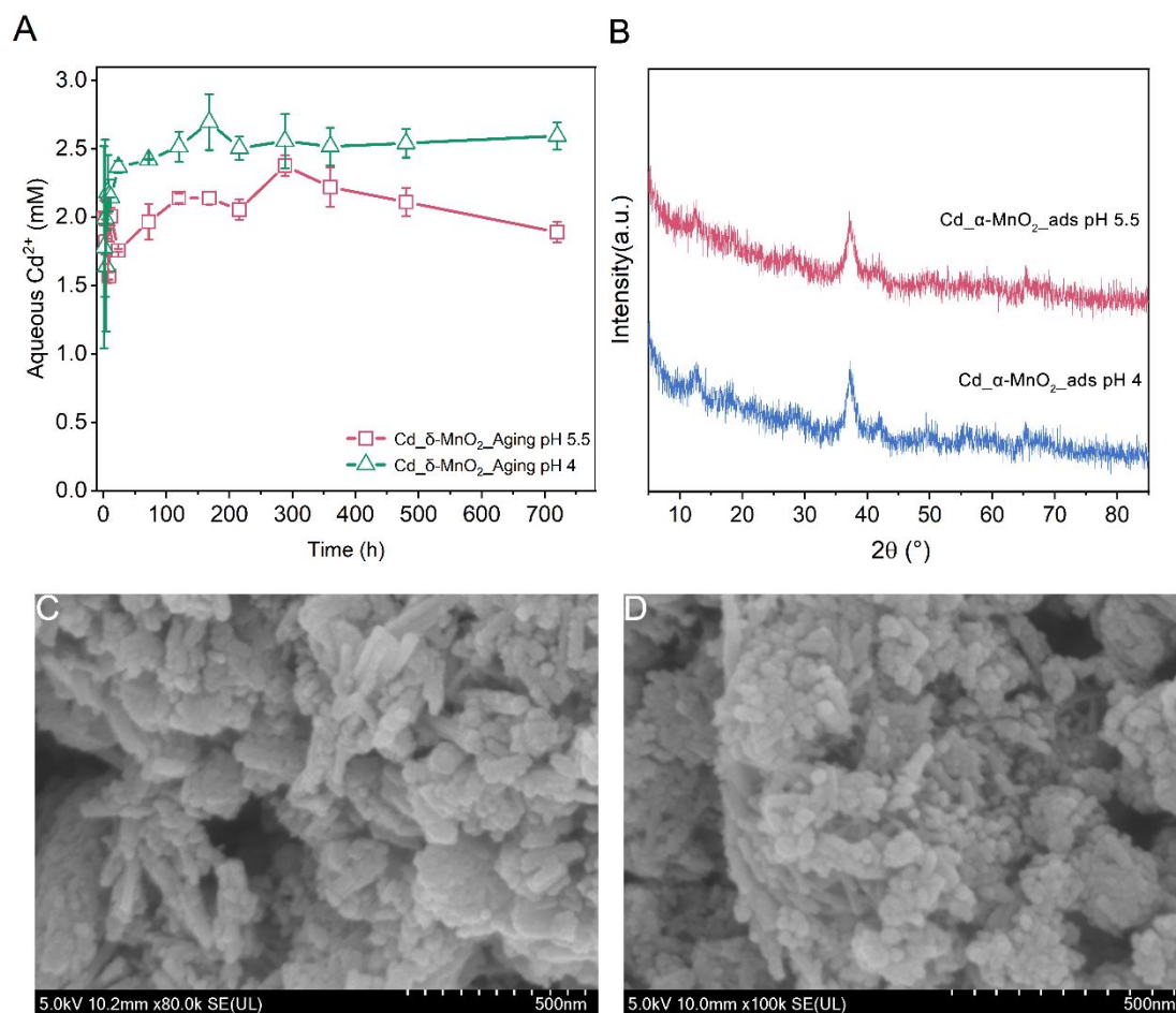
Figure S14. (A) Dynamics of aqueous \text{Cd}^{2+} concentration change during \text{Mn}^{2+} -induced \delta\text{-MnO}_2 aging in the presence of \text{Cd}^{2+} at pH 4 and 5.5; (B) XRD patterns of \text{Cd-}\alpha\text{-MnO}_2\text{-ads} solid samples at pH 4 and 5.5; (C, D) SEM images of \text{Cd-}\alpha\text{-MnO}_2\text{-ads} samples at pH 4 and 5.5.
