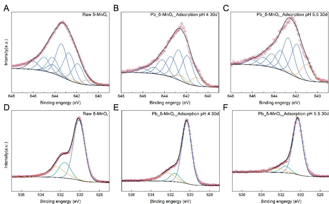
Figure S9. Mn 2p 2/3 spectra of (A) raw \delta -MnO 2 , (B) \delta -MnO 2 adsorb Pb 2+ at pH 4.0 about 30-days and (C) \delta -MnO 2 adsorb Pb 2+ at pH 5.5 about 30-days, the black solid line representing the fitted curves, the red circles line representing the XPS measurement data, blue lines for Mn(IV) fitting, and green line for Mn(III) fitting; O1s spectra of (D) raw \delta -MnO 2 , (E) \delta -MnO 2 adsorb Pb 2+ at pH 4 about 30-days and (F) \delta -MnO 2 adsorb Pb 2+ at pH 5.5 about 30-days, with the black solid line representing the fitted curves, the red circles line representing the measurement data, blue line for O 2- fitting, green line for OH - fitting, and orange line for H 2 O fitting, respectively.
