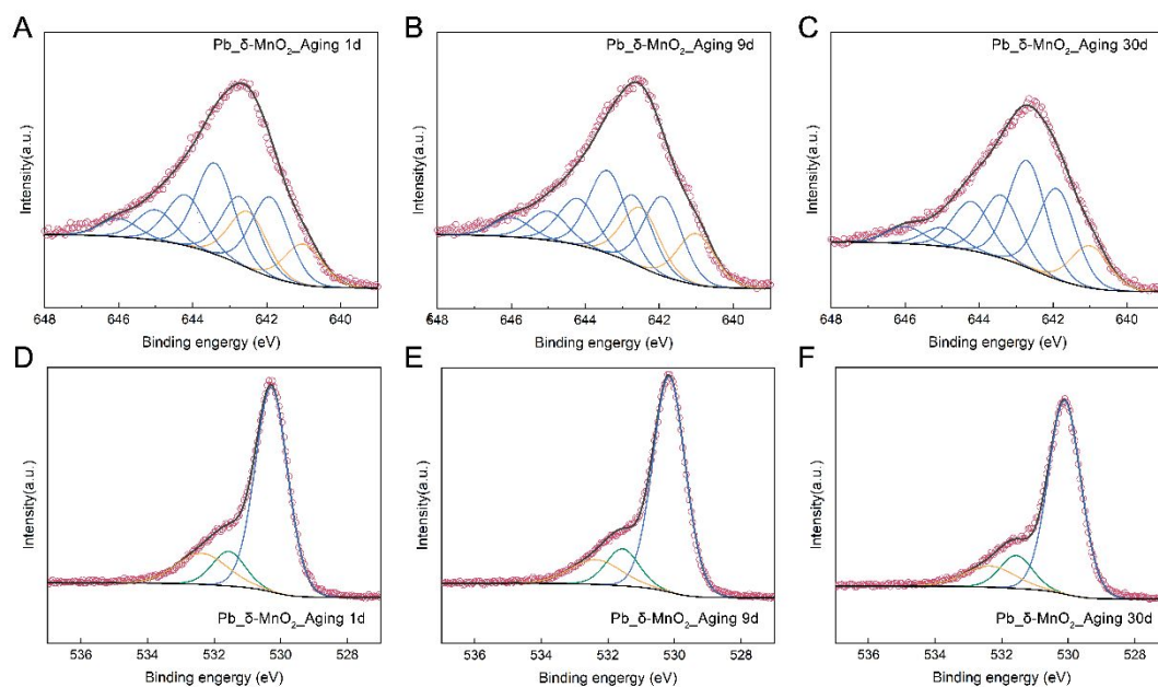
Figure S13. (A–C) Mn 2p 2/3 spectra of Mn 2+ -induced \delta -MnO 2 aging samples in the presence of Pb 2+ at pH 5.5 collected at different time intervals (i.e., 1 day, 9 days, and 30 days), with the black solid line representing the fitted curves, the red circles line representing the XPS measurement data, blue lines for Mn(IV) fitting, and orange line for Mn(III) fitting; (D–F) O1s spectra of the same samples collected at different time intervals, with the black solid line representing the fitted curves, the red circles line representing the measurement data, blue line for O 2- fitting, green line for OH - fitting, and orange line for H 2 O fitting, respectively.
