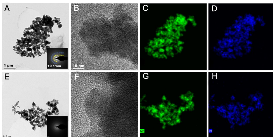
Figure S12. STEM images of Pb_ \delta -MnO 2 _ads sample at pH 4 (TEM: A; HRTEM: B) and STEM-EDS mapping image of Mn(C) and Pb (D), the inset image is SAED pattern; STEM images of Pb_ \delta -MnO 2 _ads sample at pH 5.5 (TEM: E; HRTEM: F) and STEM-EDS mapping image of Mn (G) and Pb (H), the inset image is SAED pattern.
