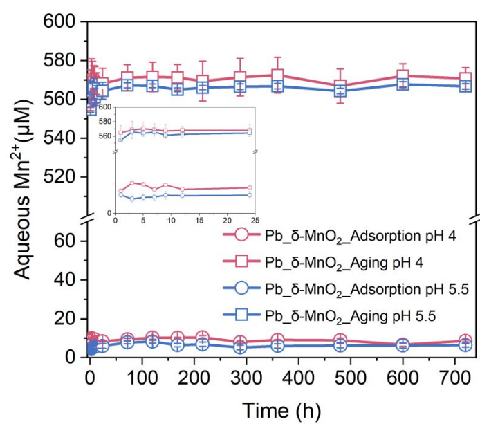
Figure S2. (A) Dynamics of dissolved Mn^{2+} concentration change during Pb^{2+} adsorption on \delta-MnO_2 and Mn^{2+} -induced \delta-MnO_2 aging in the presence of Pb^{2+} at pH 4 and 5.5.
