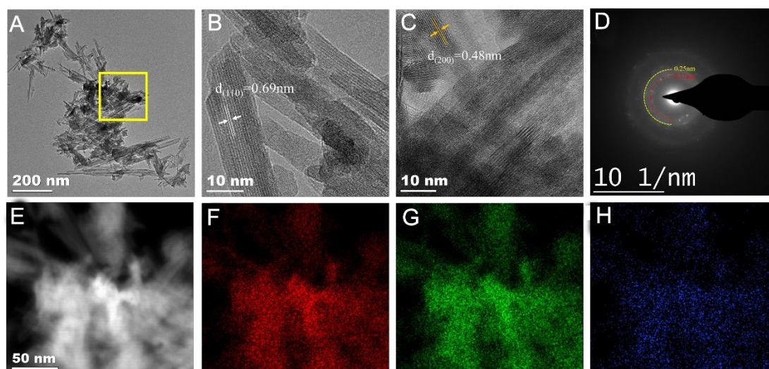
Figure S5. TEM images of Pb_α-MnO 2 _tun sample at pH 4. (A) TEM image, (B–D) HRTEM images of Pb_α-MnO 2 _tun sample along different crystal facets (B and C), and its corresponding FFT image; (E) High-magnification dark-field image of the selected yellow region in Figure S4A, (F–H) EDS mapping of O (F), Mn (G), and Pb (H) corresponding to Figure S4E.
