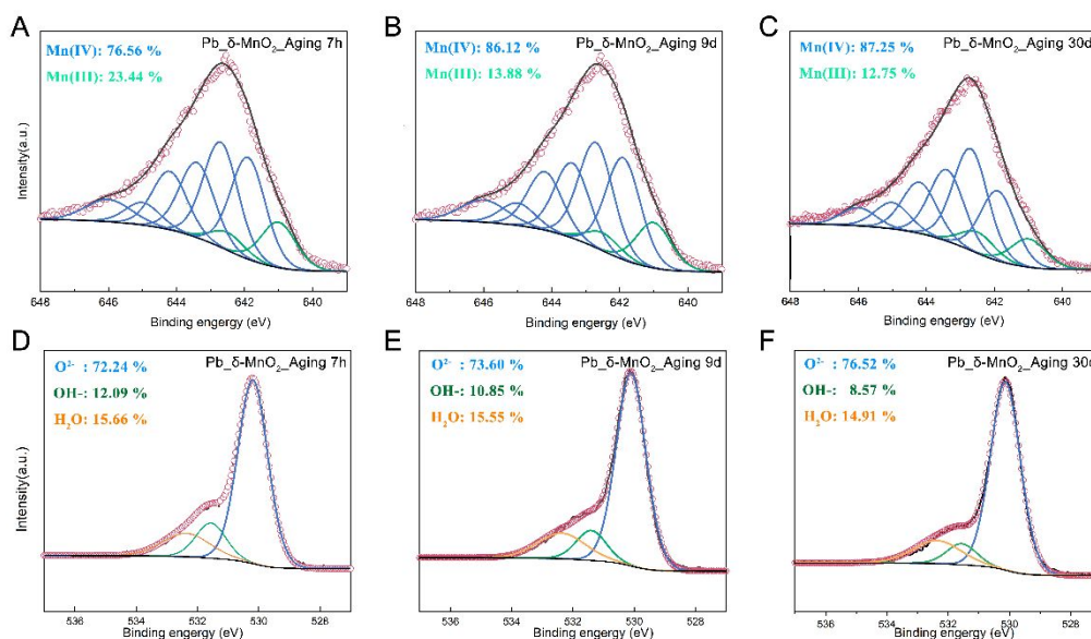
Figure S8. (A–C) Mn 2p 2/3 spectra of Mn 2+ -induced δ-MnO 2 aging samples in the presence of Pb 2+ at pH 4 collected at different time intervals (i.e., 7 hours, 9 days, and 30 days), with the black solid line representing the fitted curves, the red circles line representing the XPS measurement data, blue lines for Mn(IV) fitting, and green line for Mn(III) fitting; (D–F) O1s spectra of the same samples collected at different time intervals, with the black solid line representing the fitted curves, the red circles line representing the measurement data, blue line for O 2- fitting, green line for OH - fitting, and orange line for H 2 O fitting, respectively.
