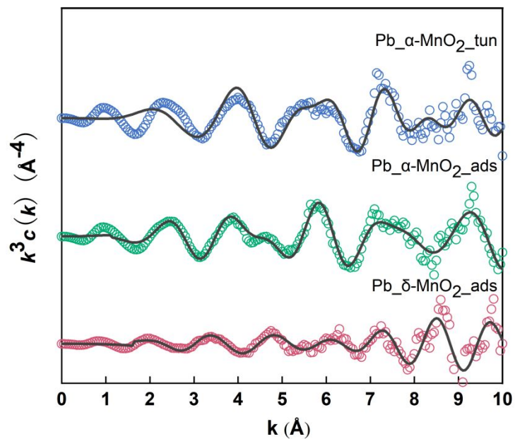
Figure S3. Pb L 3 edge EXAFS spectra of \text{Pb}_\delta\text{-MnO}_2\text{-ads} , \text{Pb}_\alpha\text{-MnO}_2\text{-tun} , and \text{Pb}_\alpha\text{-MnO}_2\text{-ads} samples from 30-day \text{Pb}^{2+} adsorption on \delta/\alpha\text{-MnO}_2 and \text{Mn}^{2+} -induced \delta\text{-MnO}_2 aging in the presence of \text{Pb}^{2+} at pH 4. The black lines represent the fitting curves, and the colorful cycles represent the XAS measurement data.
