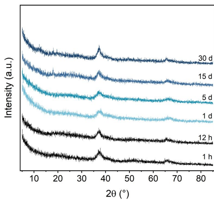
Figure S11. Time-resolved XRD patterns of solid products from Mn 2+ -induced \delta -MnO 2 aging samples at pH 5.5.
