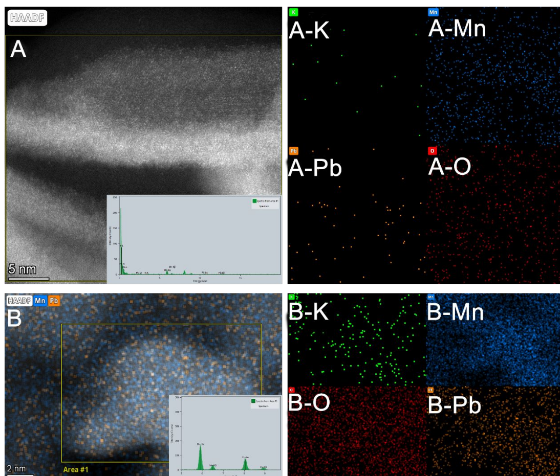
Figure S6. Elemental mapping images (Mn/Pb) collected via STEM-EDS of Pb_ \alpha -MnO 2 _tun sample at pH 4. (A) Side view of Mn oxide nanorod. The A-K, Mn, Pb, and O correspond to the elemental distributions of K, Mn, Pb, and O for image (A) Mn oxides; (B) End view of Mn oxide nanorod. B-K, Mn, Pb, and O correspond to the elemental distributions of K, Mn, Pb, and O within the yellow rectangle in image (B) Mn oxides.
