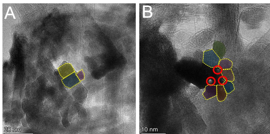
Figure S10. HRTEM image (A and B) of \text{Pb}_\alpha\text{-MnO}_2 sample. The yellow dashed lines highlight the oriented attachment of single nanorods along their side surface (A, B); The red circles in Figure S13B indicate the voids formed after the oriented assembly, leading to the sample rising to form the nanotube morphology.
