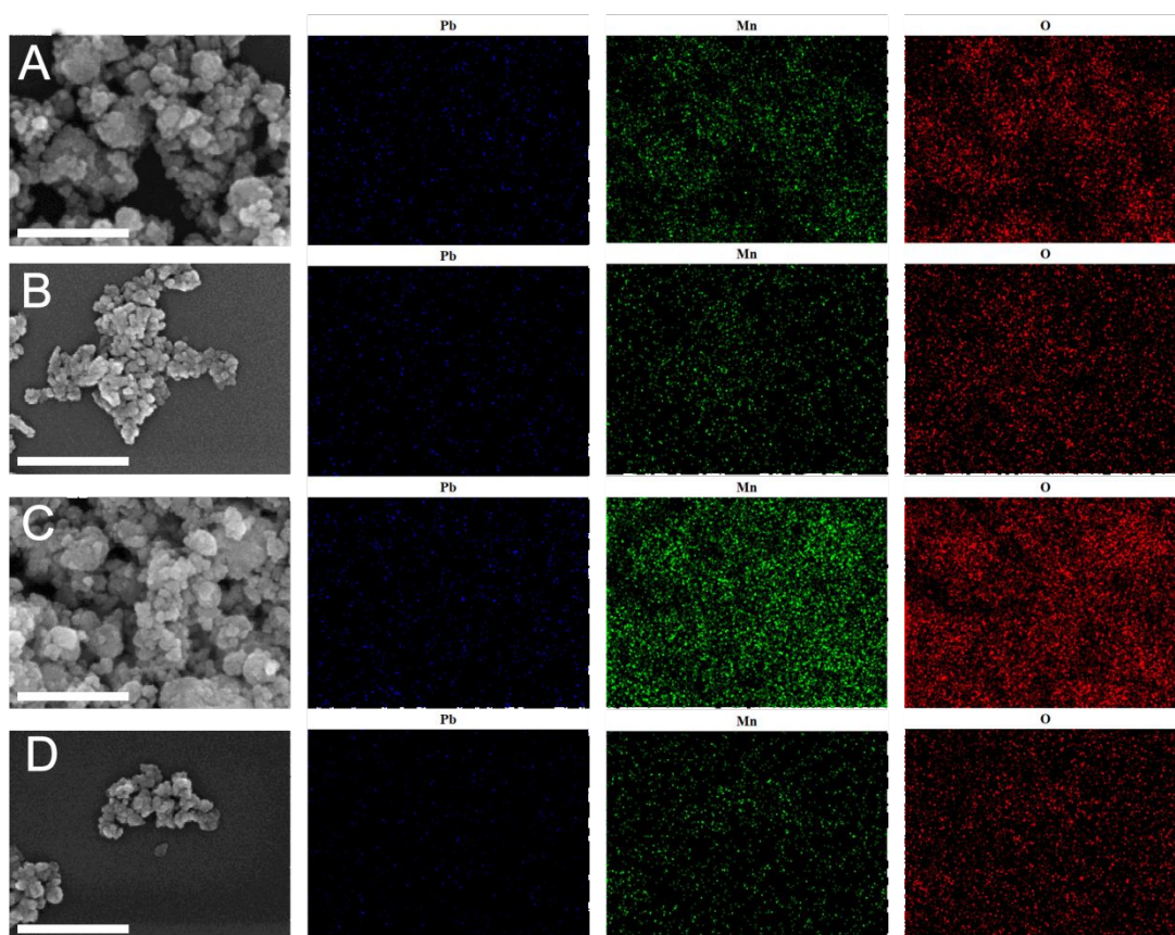
Figure S1. The SEM and EDS images (blue: Pb, green: Mn, red: O) of (A) Pb \delta -MnO _2 _ads sample at pH 4; (B) Pb \alpha -MnO _2 _tun sample at pH 4; (C) Pb \delta -MnO _2 _ads sample at pH 5.5; (D) Pb \alpha -MnO _2 _tun sample at pH 5.5. The scale bar indicates 500 nm.
