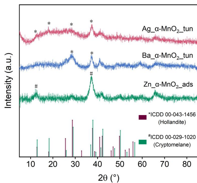
Figure S16. XRD patterns of 7-day \text{Mn}^{2+} -induced \delta\text{-MnO}_2 transformation samples in the presence of \text{Ag}^+ , \text{Ba}^{2+} , or \text{Zn}^{2+} at pH 4.
