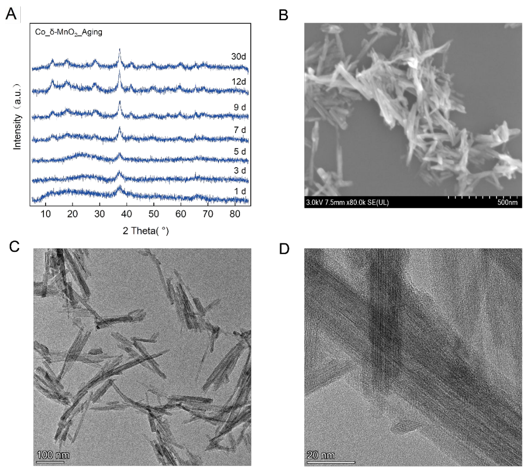
Figure S15. (A) Time-resolved XRD patterns of solid products from Mn 2+ -induced \delta -MnO 2 aging in the presence of Co 2+ at pH 4 collected at different time intervals; (B) The SEM image of Co- \alpha -MnO 2 sub sample at pH 4; (C, D) The TEM and HRTEM images of Co- \alpha -MnO 2 sub sample at pH 4.
