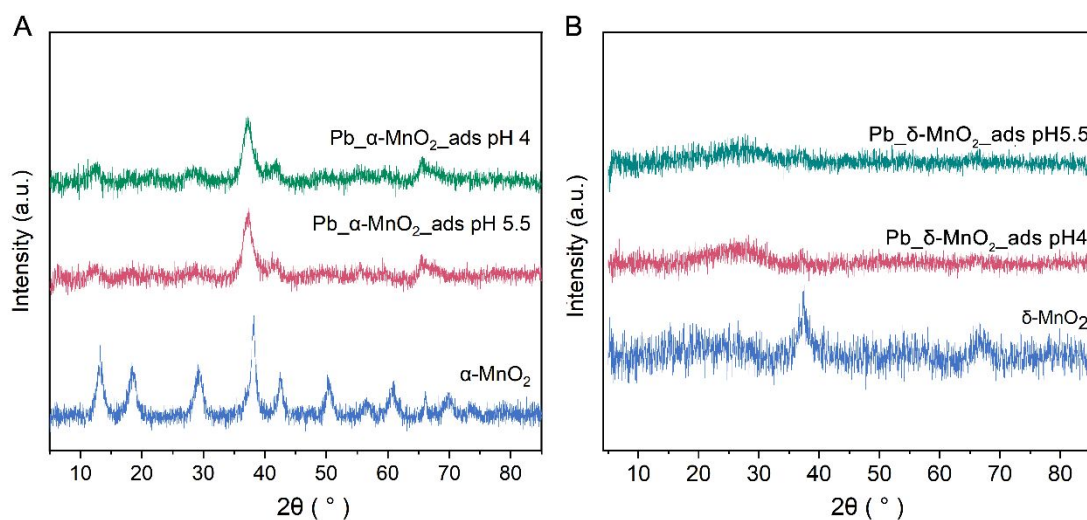
Figure S7. (A) XRD patterns of \alpha -MnO 2 samples after 30-day Pb 2+ adsorption at pH 4 and 5.5. The blue line represents the synthetic \alpha -MnO 2 sample as a reference. (B) XRD patterns of \delta -MnO 2 samples after 30-day Pb 2+ adsorption at pH 4 and 5.5. The blue line represents the synthetic \delta -MnO 2 sample as a reference.
