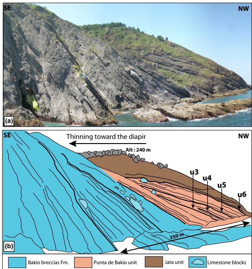
Fig. 6. (a) Westward view of the Punta de Bakio sedimentary wedge. (b) Interpretation of the wedge, composed from bottom to top of the Bakio breccias Fm., Punta de Bakio and Jata units. These units exhibit a westward decreasing dip and the Punta de Bakio unit displays four angular unconformities (u3 to u6, Fig. 5). Near the diapir contact, beds are overturned (about 10 m to the east of the picture).
