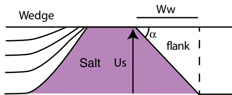
Fig. 5. Simple model of salt rise used to estimate salt height from the dip angle along the flanks, where U_s is the height of salt after diapir growth (or differential vertical displacement), \alpha the tilt angle in the wedge and W_w the width of the wedge.
