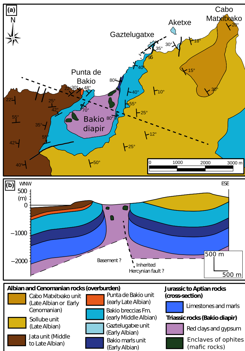
Fig. 3. (a) Geological map of the Bakio area and, (b) cross-section through the Bakio diapir, based on new field work and data from Robles et al. (1988) and Robles et al. (1989), García-Mondéjar & Robador (1986–1987), Pujalte et al. (1986–1987), Vicente-Bravo & Robles (1991a,b). The dotted line indicates the location of the cross-section.
