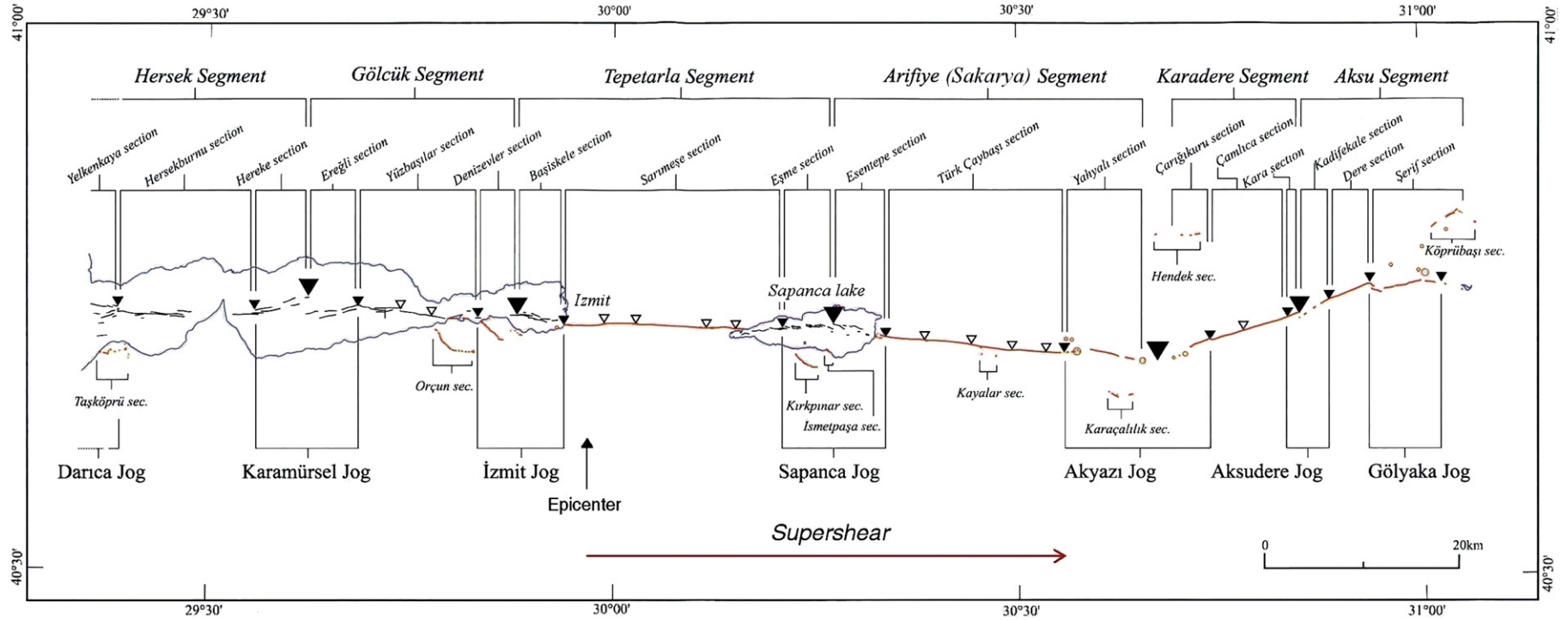
Segment structure of the surface rupture of the August 17, 1999 İzmit earthquake
